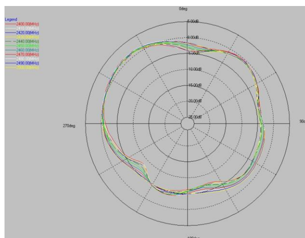
2.4G phi=90deg
