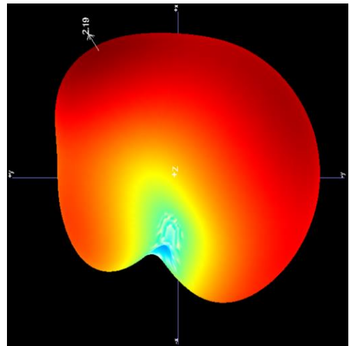
2.4G 3D
