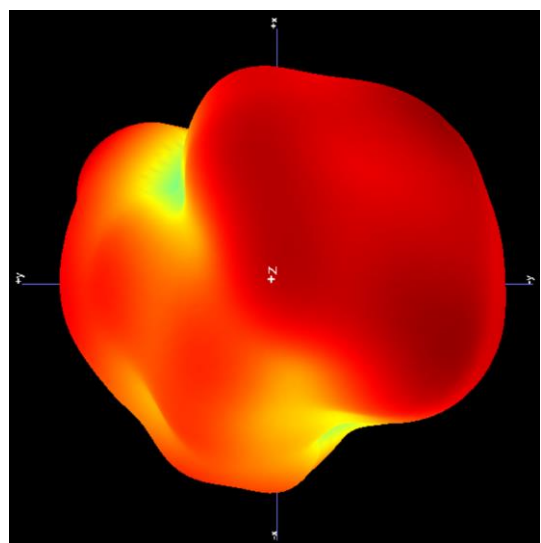
5G 3D
