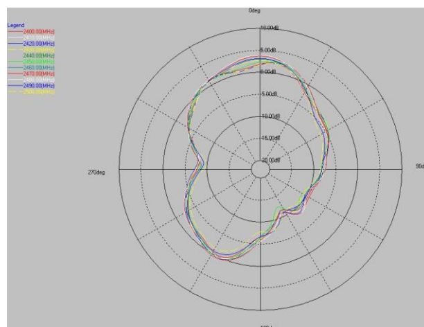
2.4G phi=90deg
