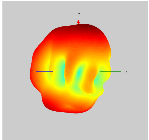
2.4G 3D
