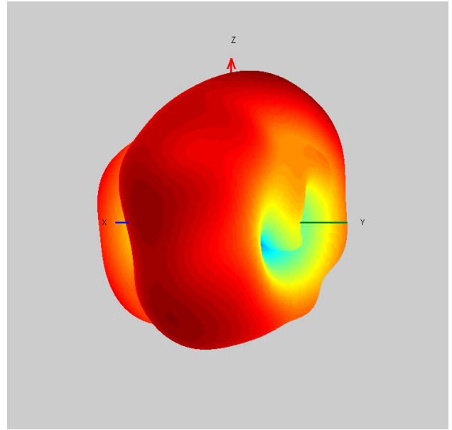
5G 3D
