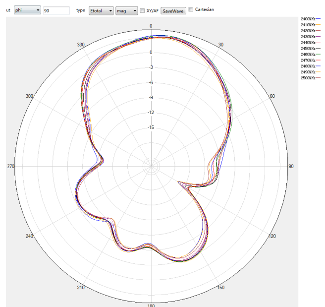
2.4G phi=90deg
