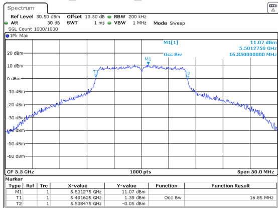
802.11a_5500MHz_Chain 0 16.850MHz
