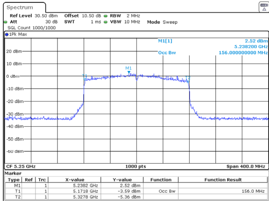
802.11ax160_5250MHz_RU_Full_Chain 1 156MHz
