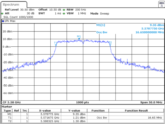
802.11a_5580MHz_Chain 2 16.650MHz
