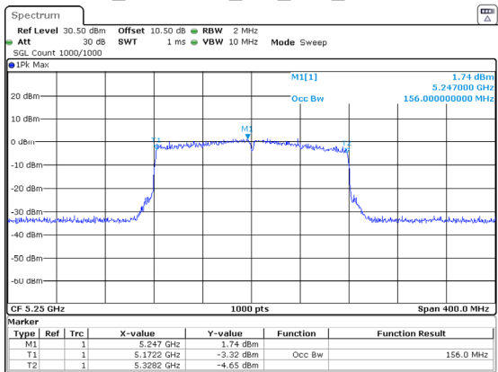
802.11ax160_5250MHz_RU_Full_Chain 0 156MHz
