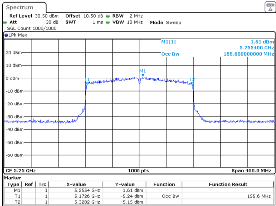
802.11ax160_5250MHz_RU_Full_Chain 2 155.600MHz
