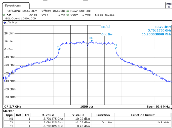
802.11a_5700MHz_Chain 0 16.900MHz
