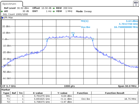
802.11a_5700MHz_Chain 1 16.750MHz
