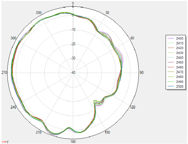
2.4G phi=90deg
