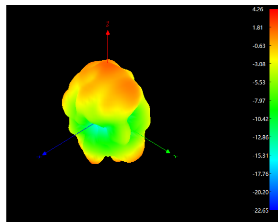
5G 3D
