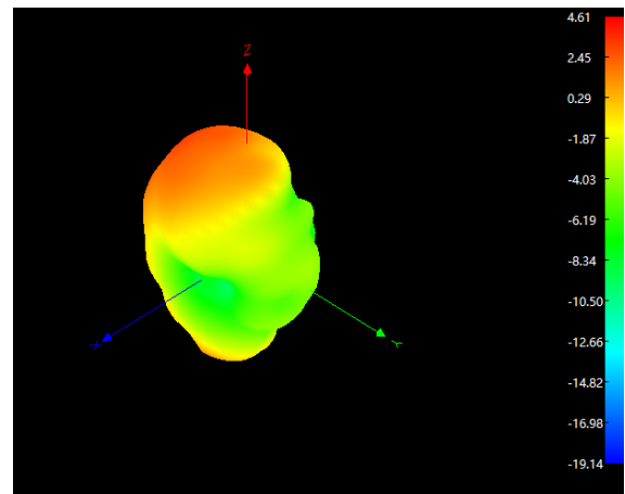
2.4G 3D
