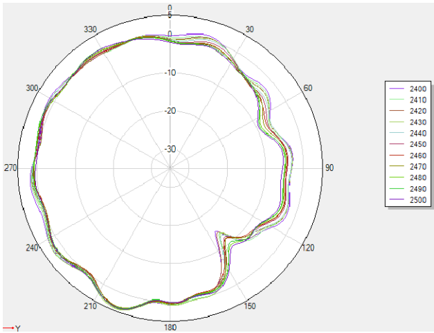
2.4G phi=90deg
