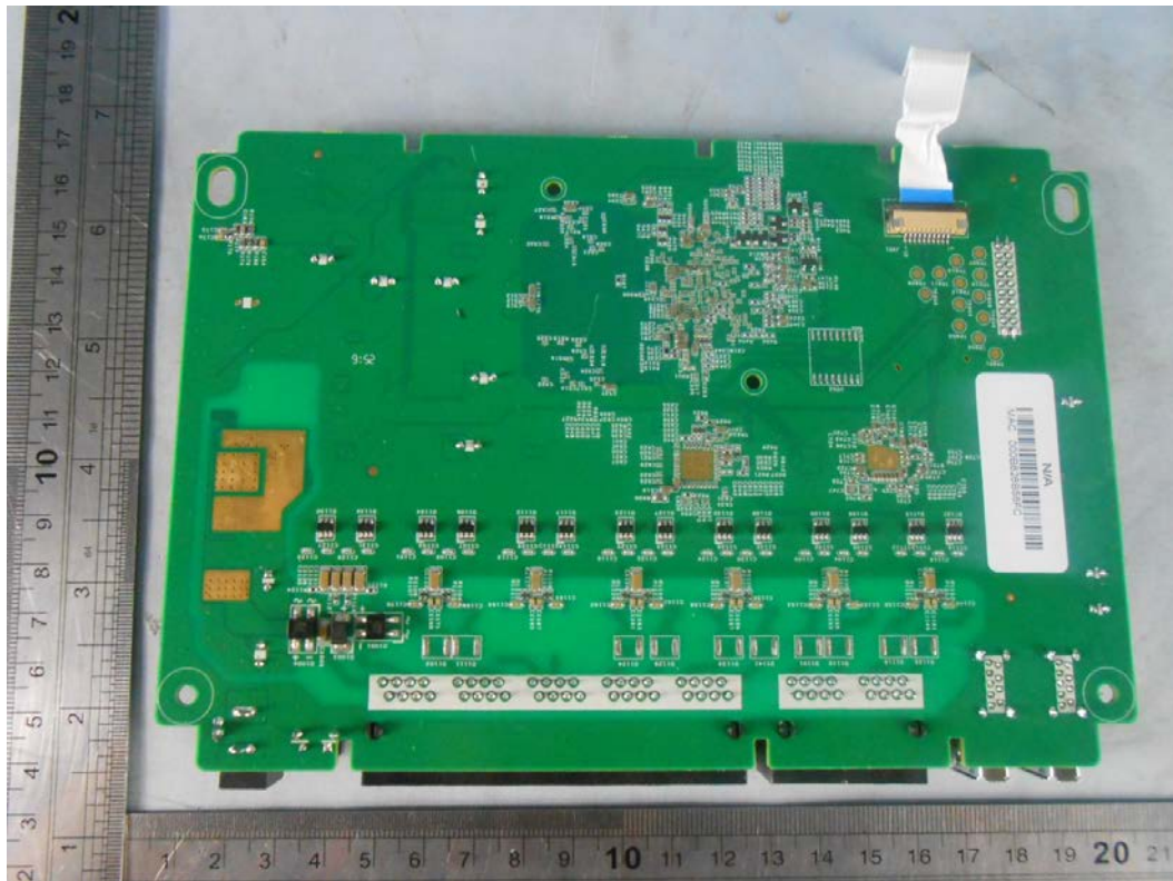
Mainboard-Bottom view -01
