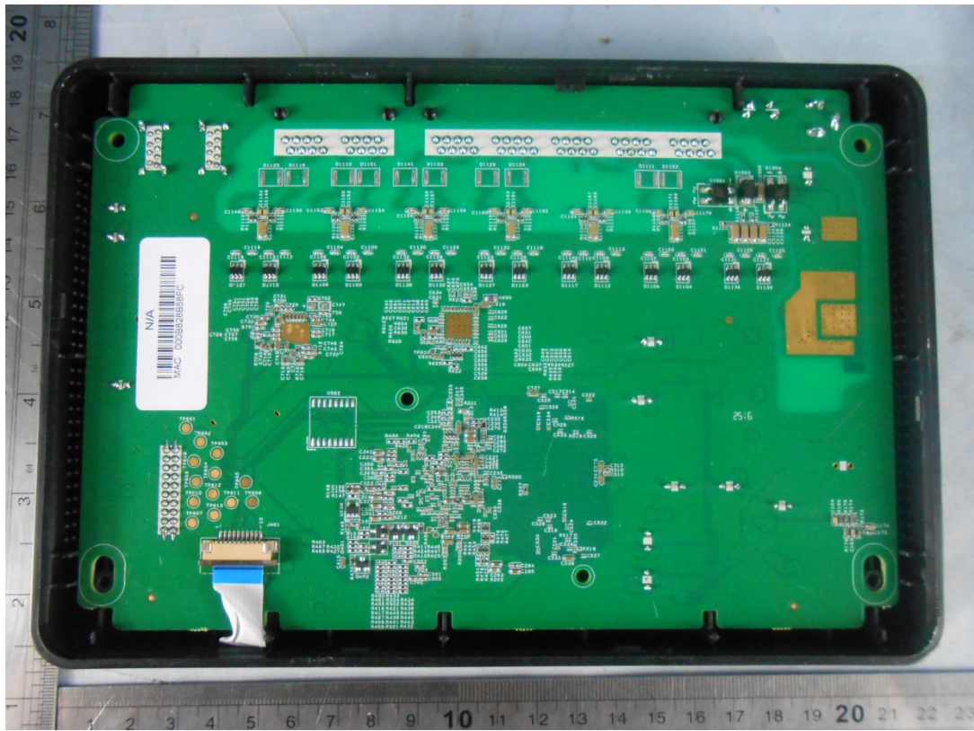
EUT-Uncovered View
