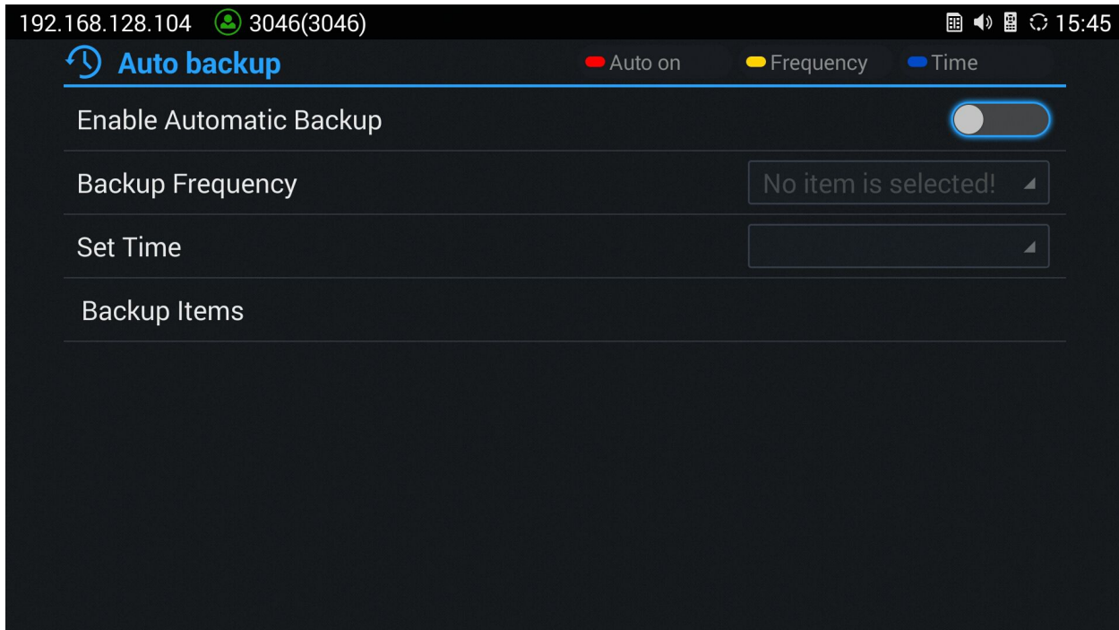
Figure 41 Backup Screen
