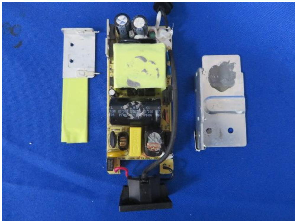
(6) EUT Photo (MN: NBS65A120500M3)
