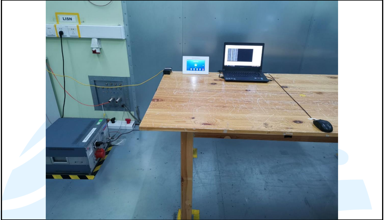
Conducted Emission Test Setup-3_Test Mode 4
