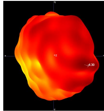
5G 3D
