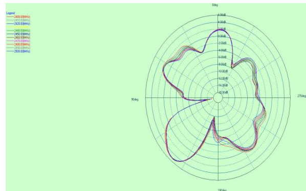
2.4G phi=90deg
