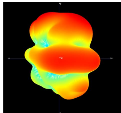
2.4G 3D
