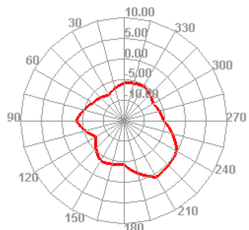
2.4G phi=90deg
