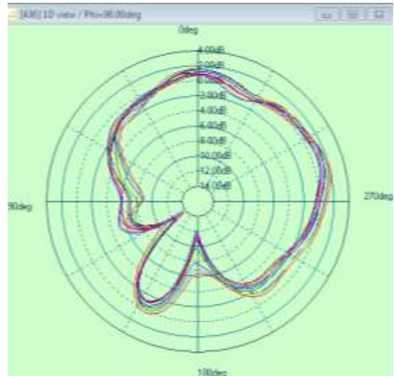
2.4G phi=90deg
