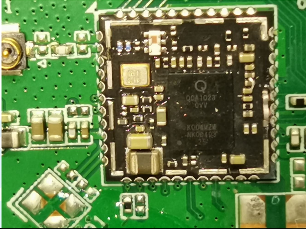
EUT Photo_ Wi-Fi Module Unshielded View
