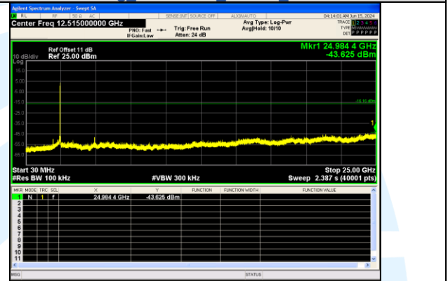
30.0 MHz - 25000.0 MHz IEEE 802.11g Channel 11 20MHz Antenna 0
