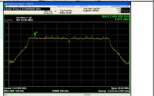
In-Band Reference Level IEEE 802.11n Channel 1 20MHz Antenna 0
