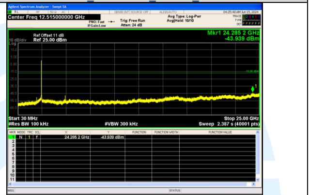
30.0 MHz - 25000.0 MHz IEEE 802.11n Channel 11 20MHz Antenna 0
