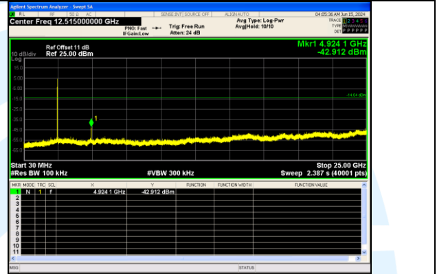
30.0 MHz - 25000.0 MHz IEEE 802.11b Channel 11 20MHz Antenna 0
