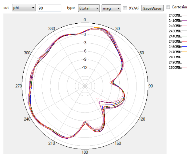
2.4G phi=90deg
