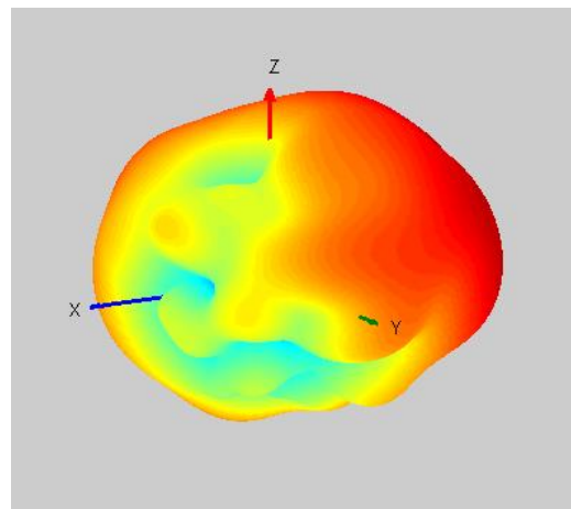
5G 3D
