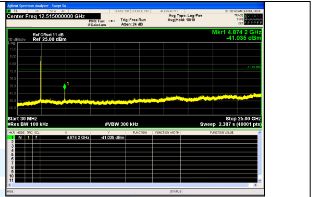
30.0 MHz - 25000.0 MHz IEEE 802.11b Channel 6 20MHz Antenna 0
