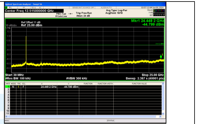
30.0 MHz - 25000.0 MHz IEEE 802.11n Channel 6 20MHz Antenna 0
