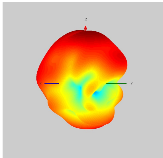
5G 3D
