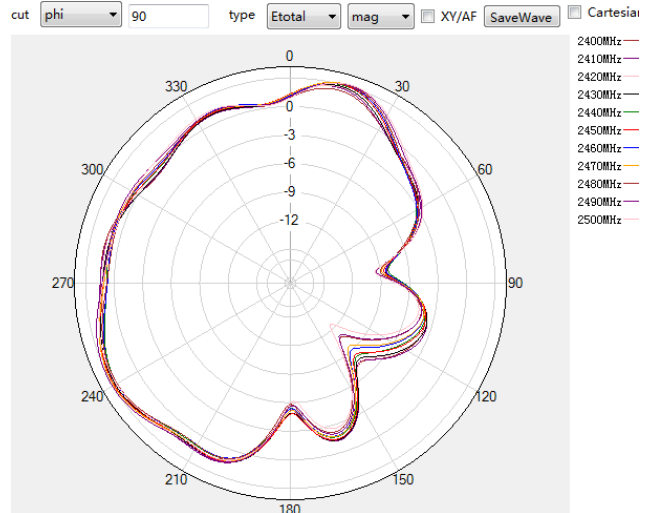
2.4G phi=90deg
