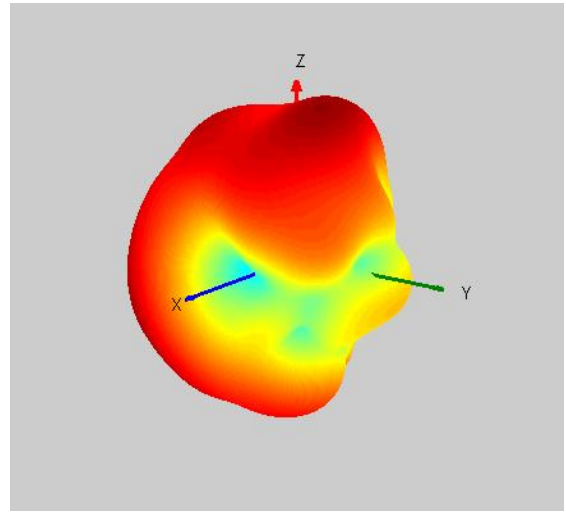
2.4G 3D
