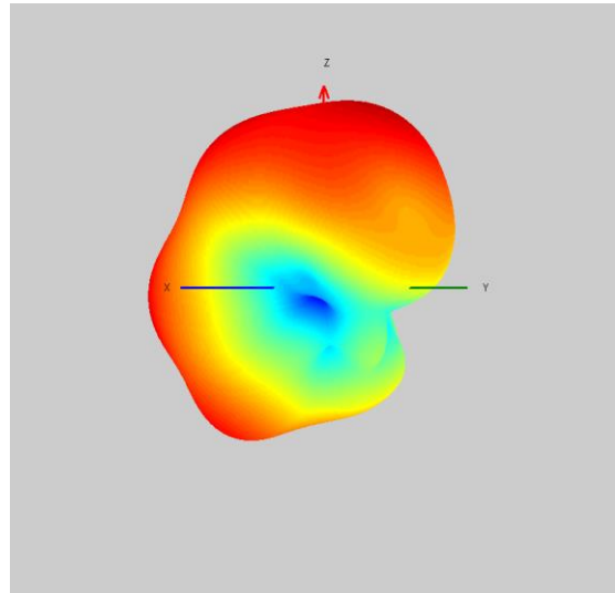
2.4G 3D
