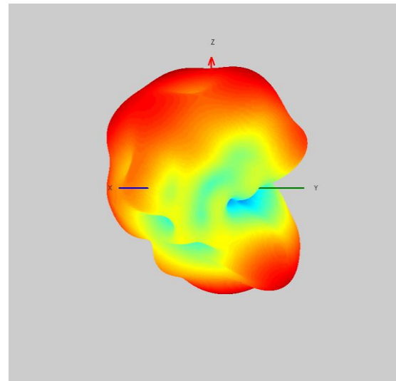
5G 3D
