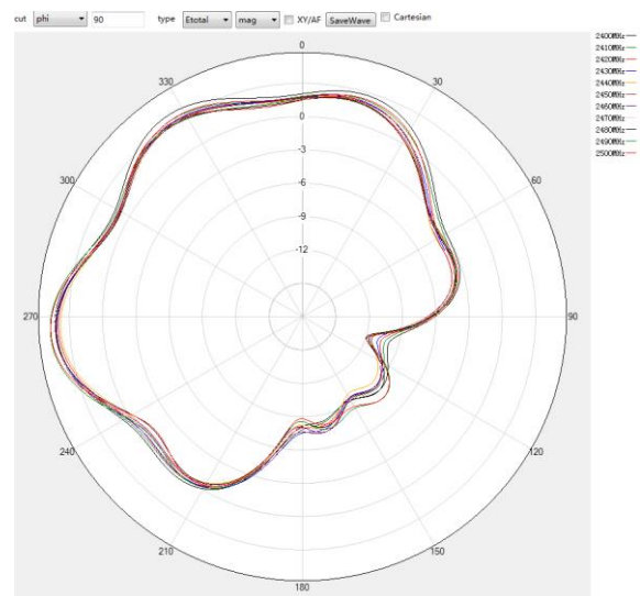
2.4G phi=90deg
