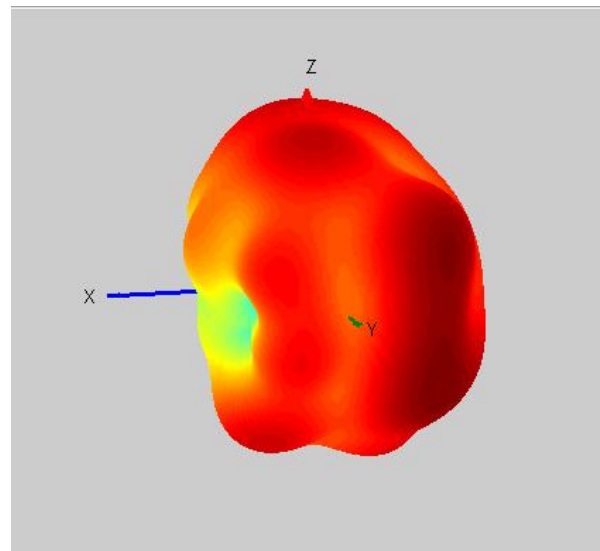
2.4G 3D
