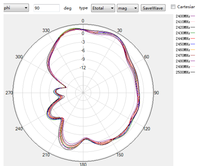
2.4G phi=90deg
