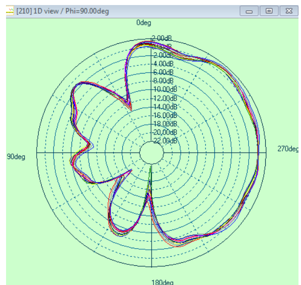
2.4G phi=90deg
