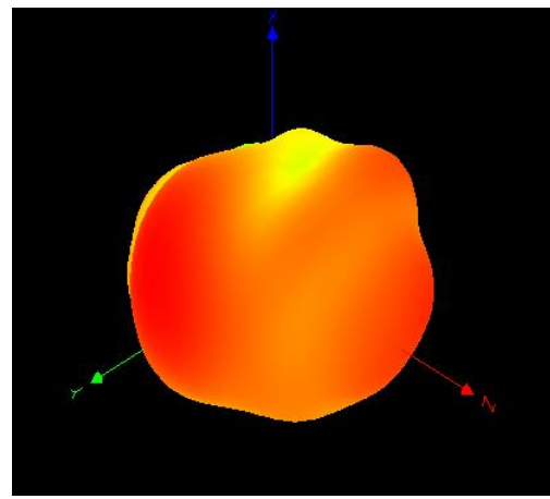
2.4G 3D
