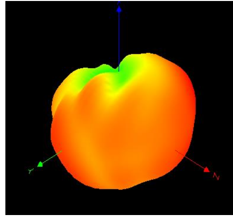
5G 3D
