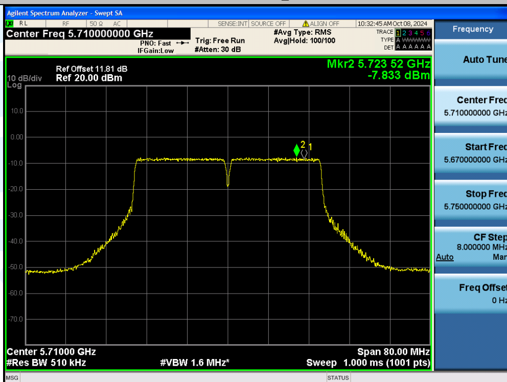
11AC40SISO-Ant1-5710_UNII-3-PASS
