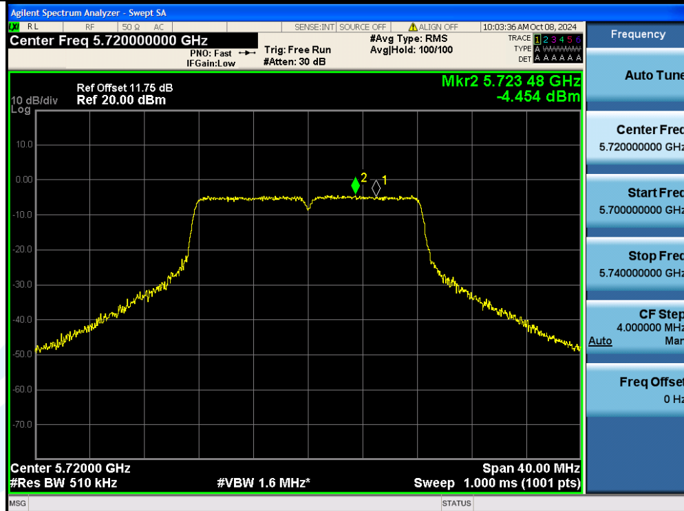
11A-Ant1-5720_UNII-3-PASS
