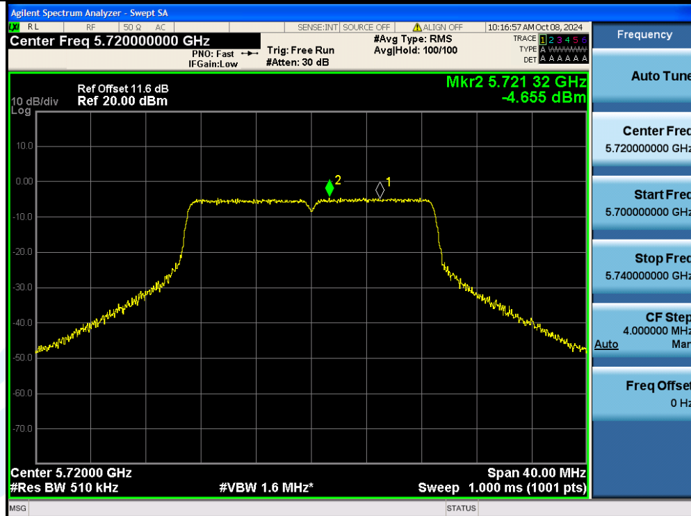
11AC20SISO-Ant1-5720_UNII-3-PASS
