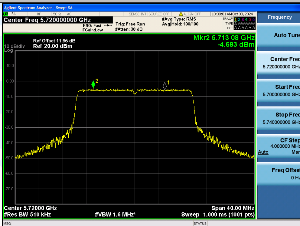
11AX20SISO-Ant1-5720_UNII-3-PASS
