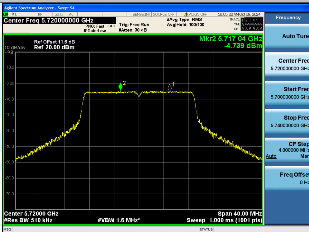
11N20SISO-Ant1-5720_UNII-3-PASS
