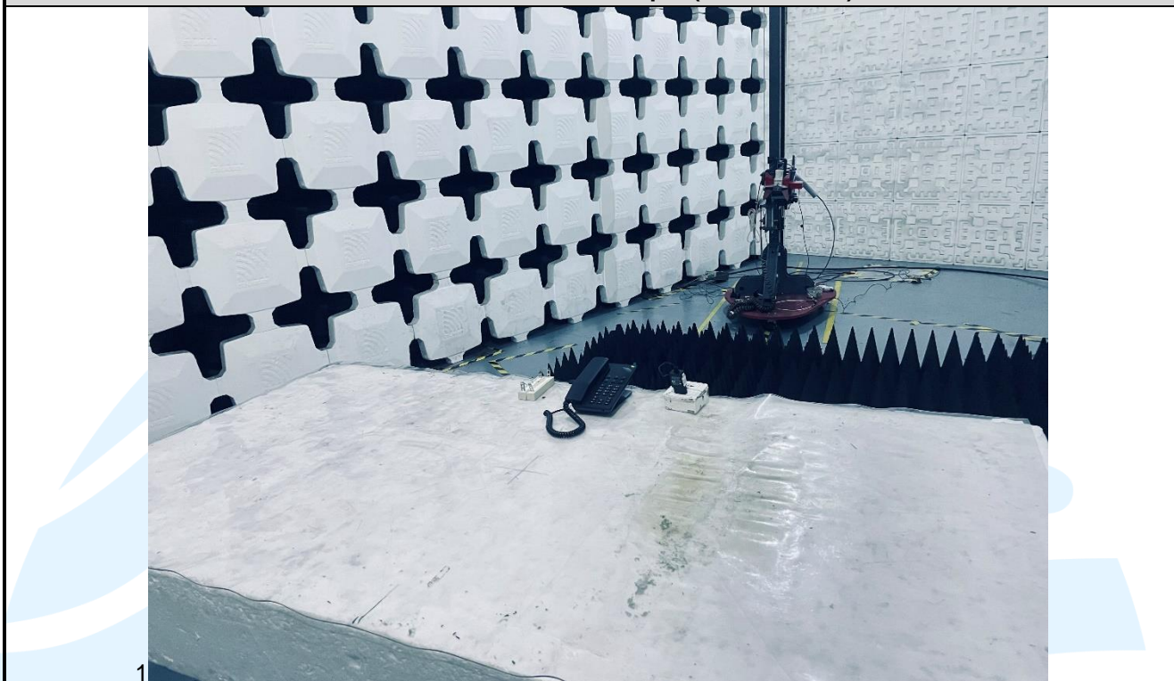
Radiated emission Test Setup-2 (Above 1 GHz)
