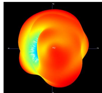
2.4G 3D
