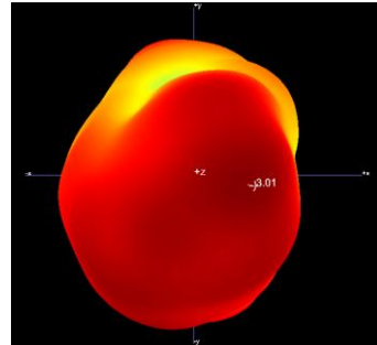
5G 3D
