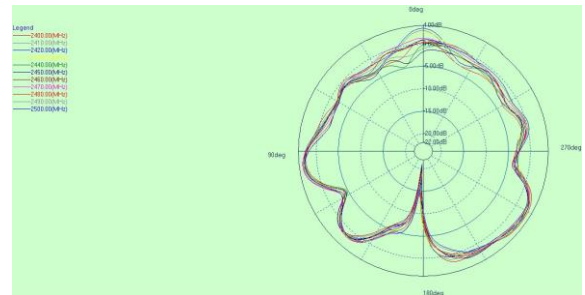
2.4G phi=90deg
