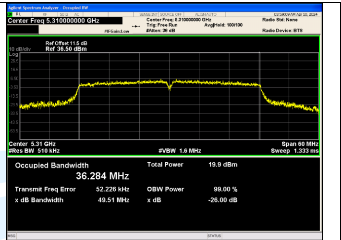
IEEE 802.11ac_Channel 62_40MHz_Antenna 2
