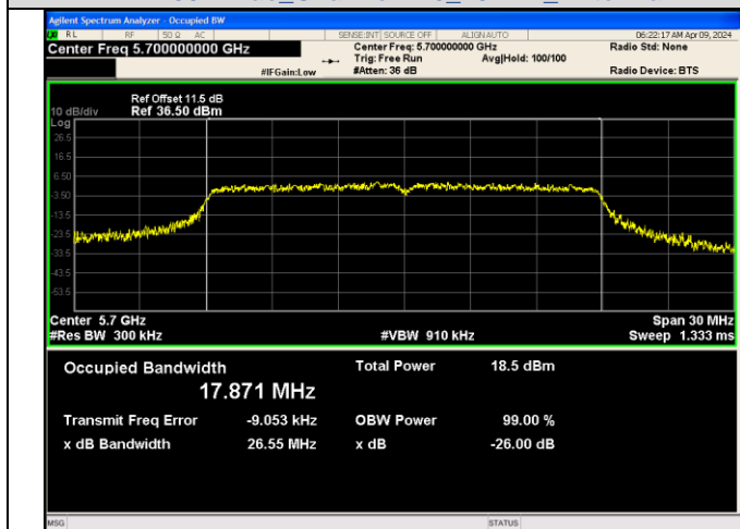
IEEE 802.11ac_Channel 140_20MHz_Antenna 0
