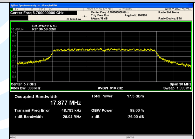
IEEE 802.11ac_Channel 140_20MHz_Antenna 1
