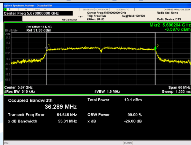
IEEE 802.11ac_Channel 134_40MHz_Antenna 2
