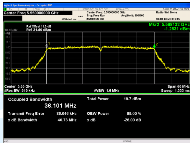
IEEE 802.11ac_Channel 110_40MHz_Antenna 2
