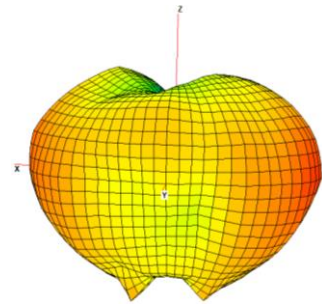
5G 3D
