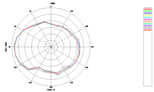
2.4G phi=90deg
