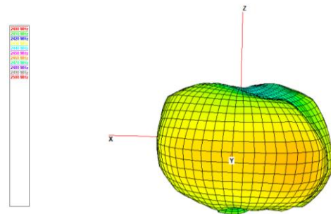
2.4G 3D
