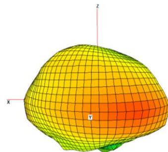
2.4G 3D
