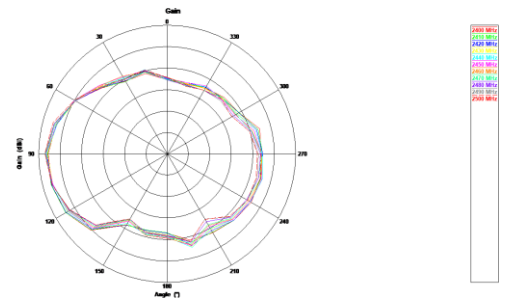
2.4G phi=90deg
