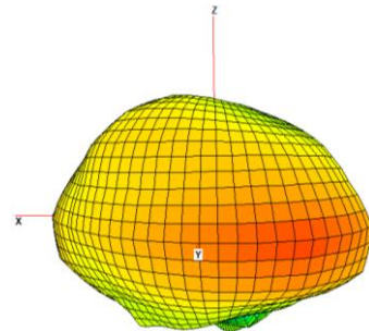
2.4G 3D
