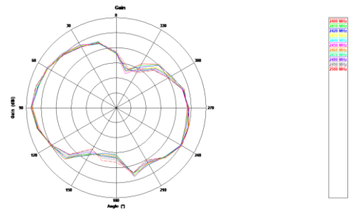
2.4G phi=90deg
