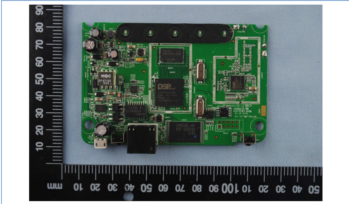
Internal Photos YZZDP760
