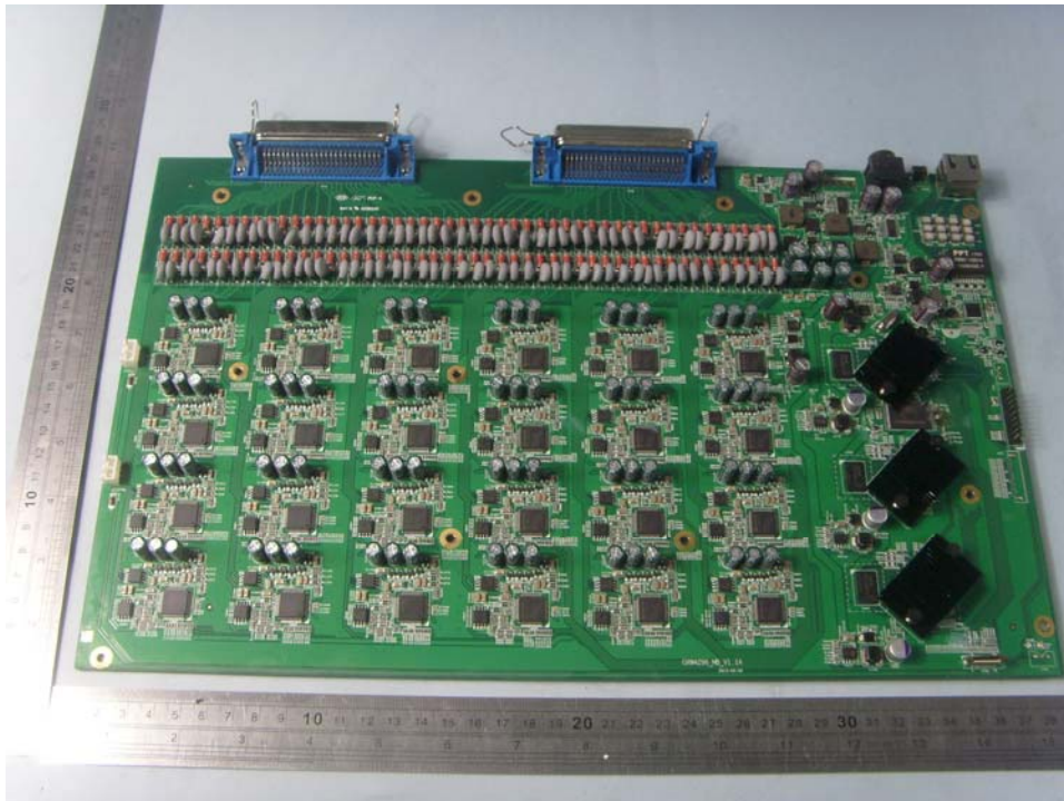
Mainboard- Top View(full view)
