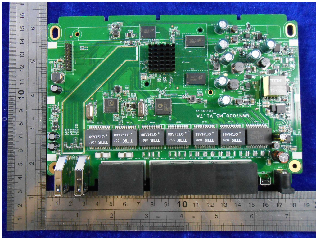
Mainboard-Top view
