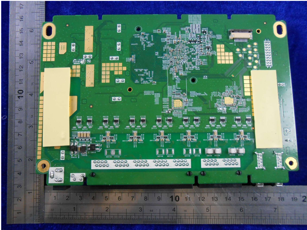
Mainboard-Bottom view
