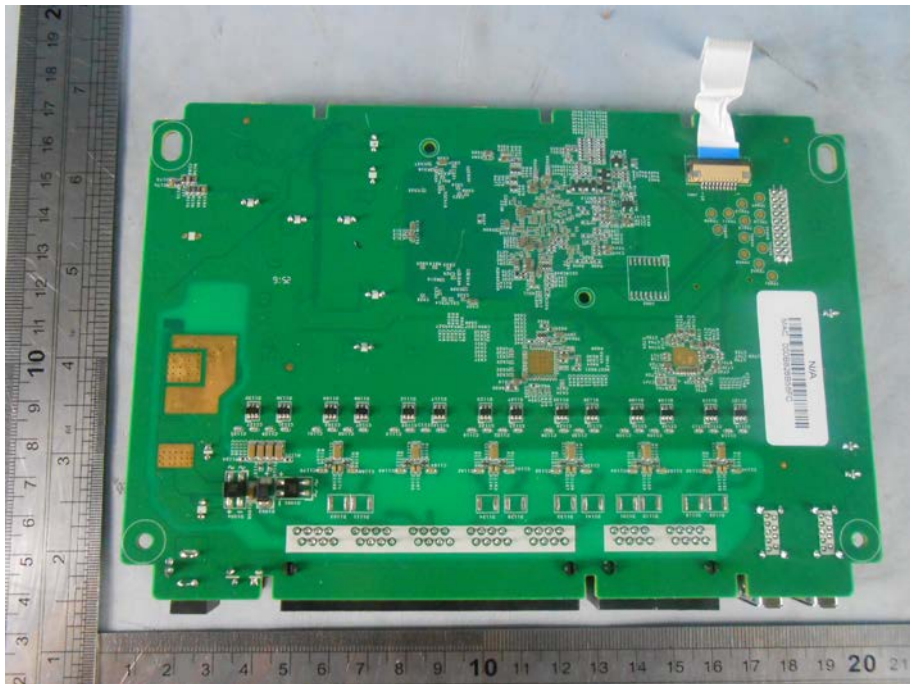
Mainboard-Bottom view
