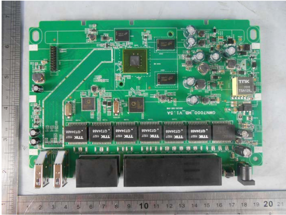
Mainboard-Top view
