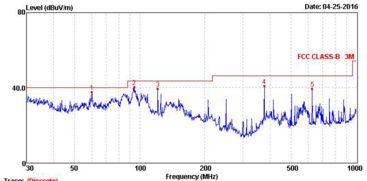
Vertical: Radiated Emission Test Plot(30-1000MHz)
