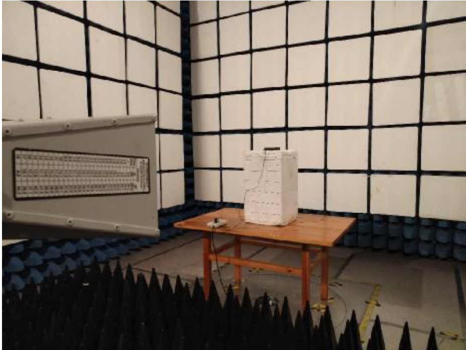
Radiated Test above 1G
