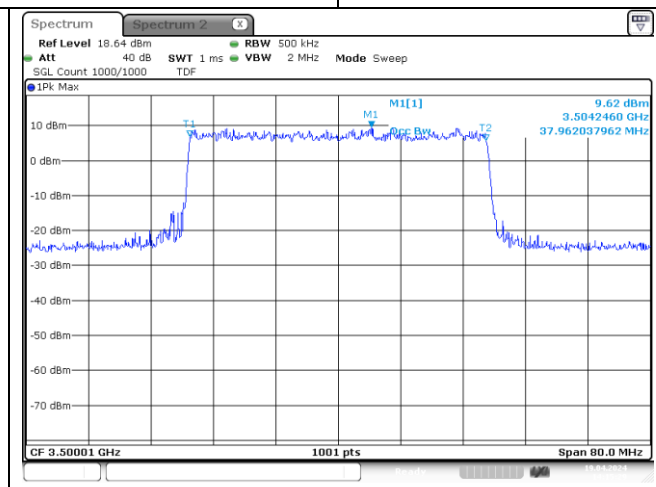
40 MHz Middle Channel CP-OFDM 16QAM
