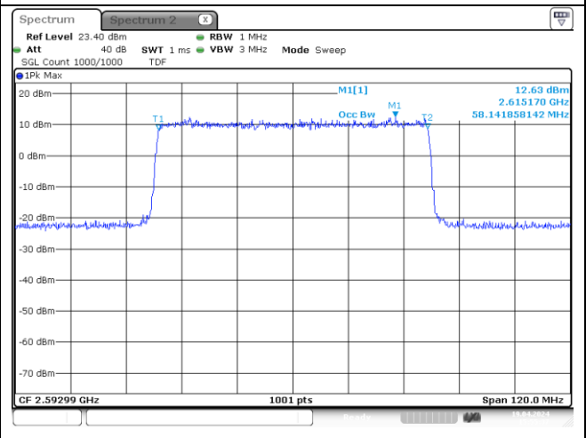
60 MHz Middle Channel CP-OFDM QPSK
