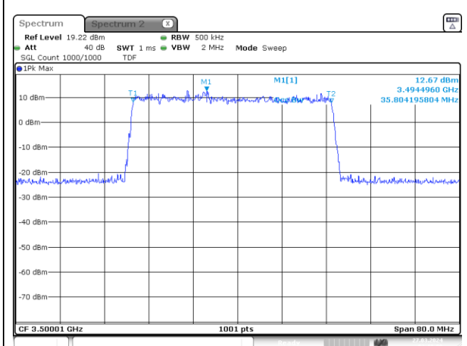
40 MHz Middle Channel DFT-S-OFDM 16QAM
