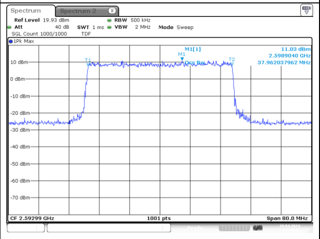
40 MHz Middle Channel CP-OFDM QPSK
