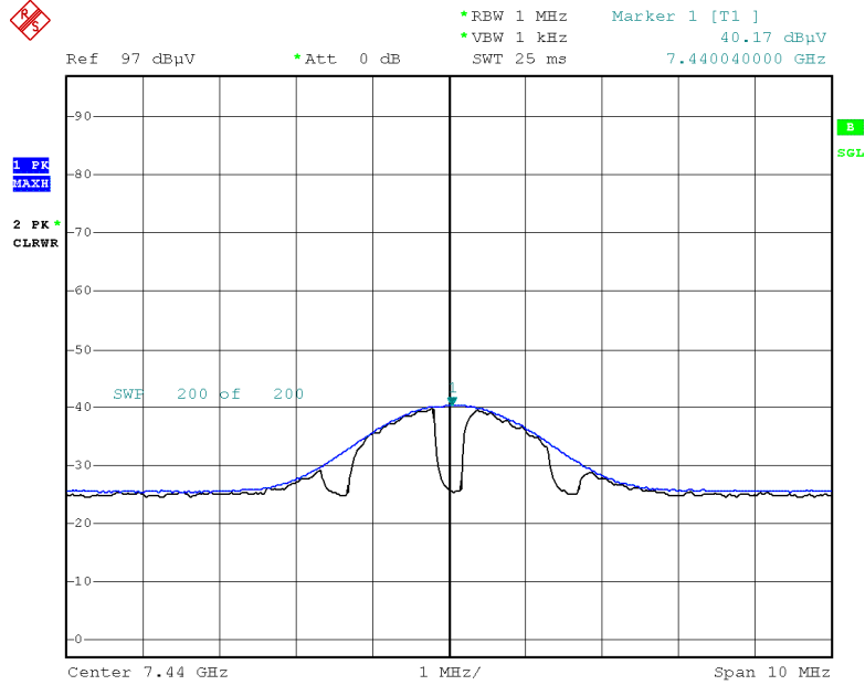
Radiated Spurious Emissions plot – Average Reading (8DPSK, Ch.78 3rd Harmonic, H)
