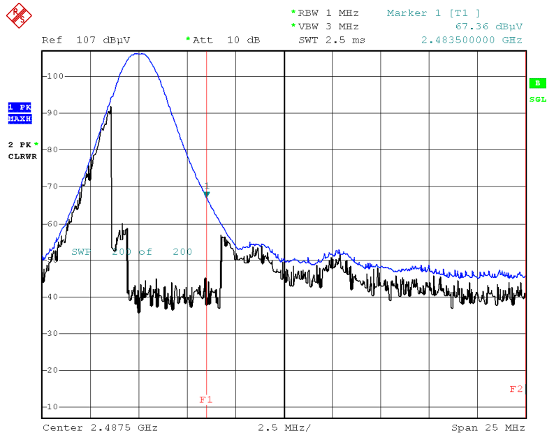
Radiated Restricted Band Edges plot –Peak Reading ( \pi/4 DQPSK, Ch.78, X-H)
