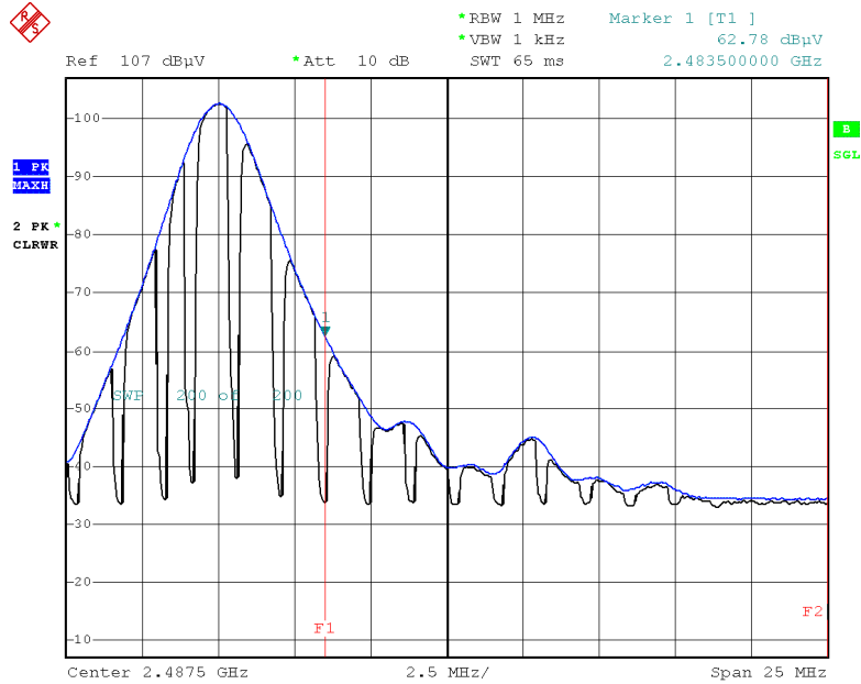
Radiated Restricted Band Edges plot – Average Reading ( \pi/4 DQPSK, Ch.78, X-H)
