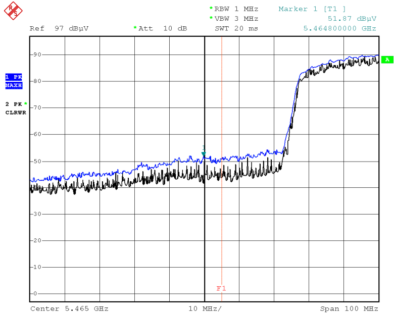
Peak Reading (802.11ac(80M), Ch.106, Z-V)
