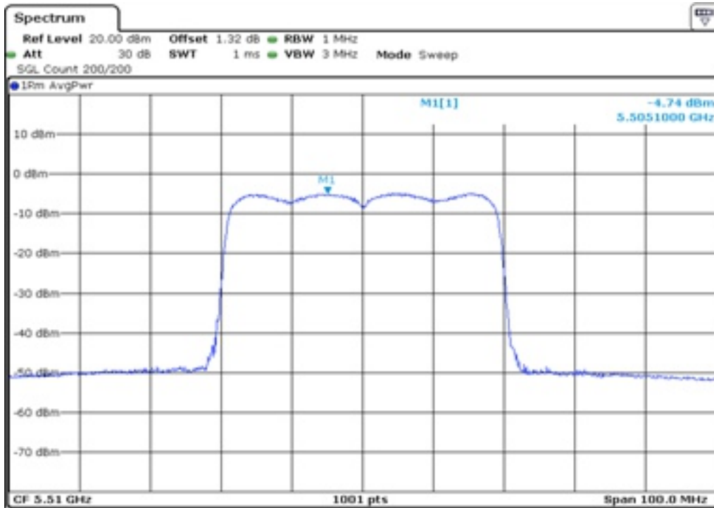
37 Peak Power Spectrul Density
