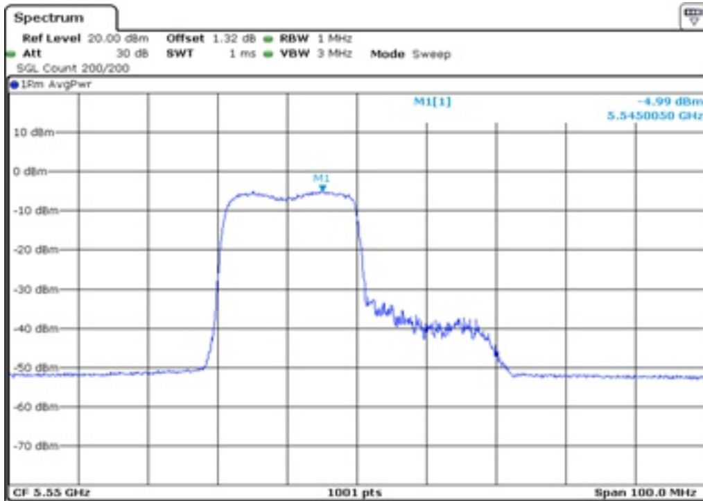
30 Peak Power Spectrul Density
