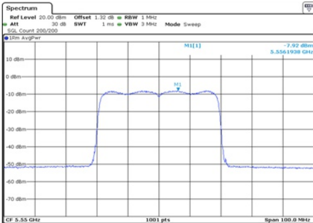
35 Peak Power Spectrul Density
