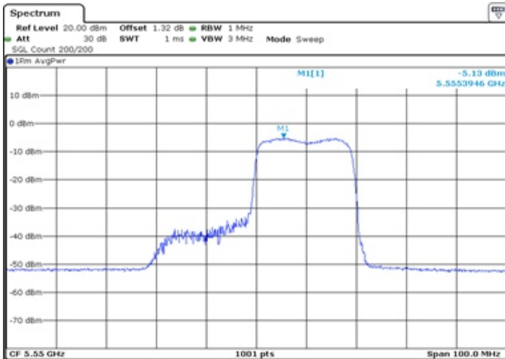
31 Peak Power Spectrul Density
