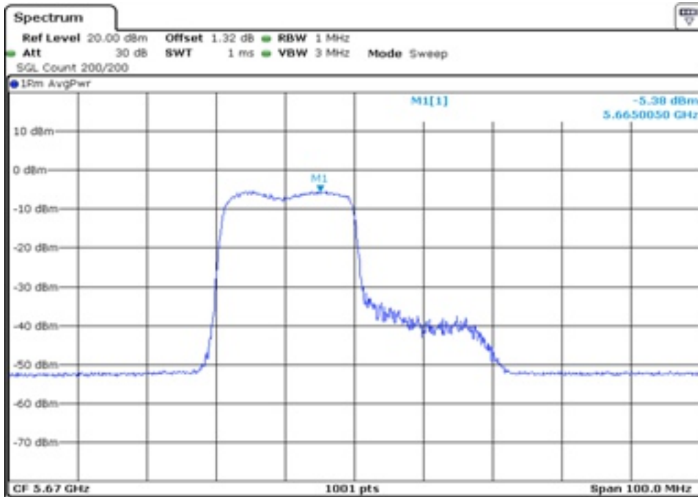
32 Peak Power Spectrul Density
