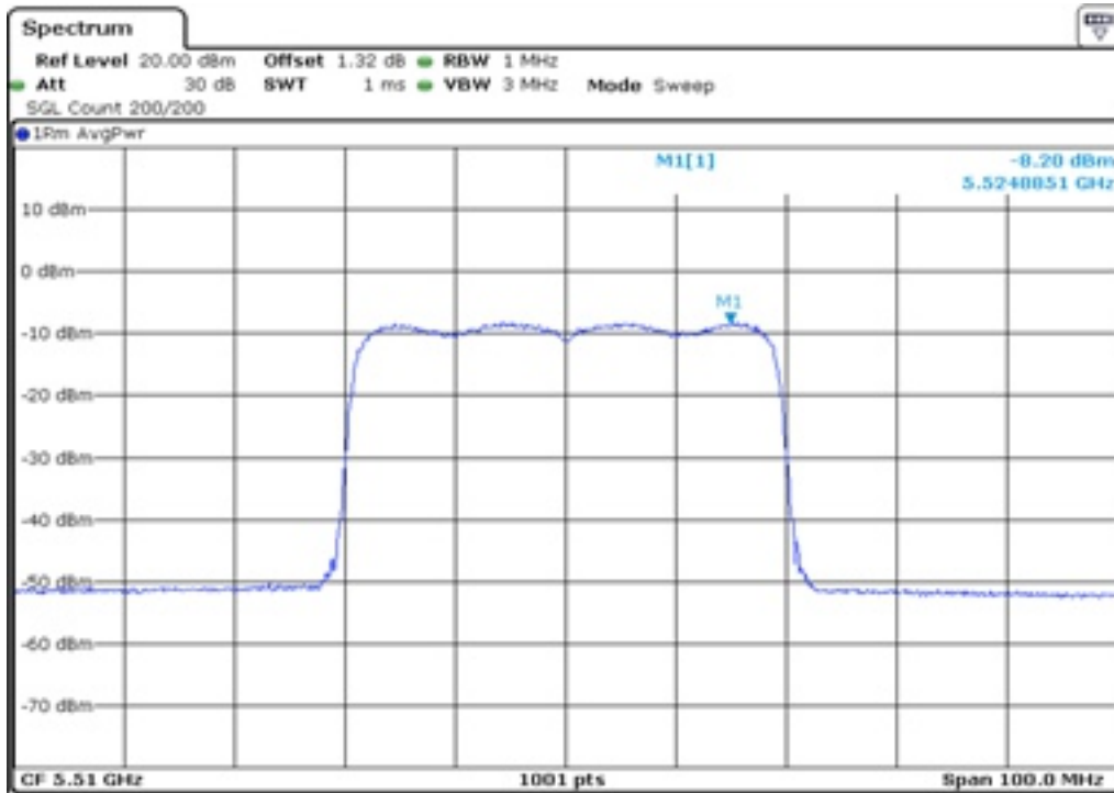
34 Peak Power Spectrul Density
