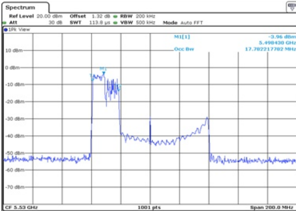
7 99% Occupied Bandwidth
