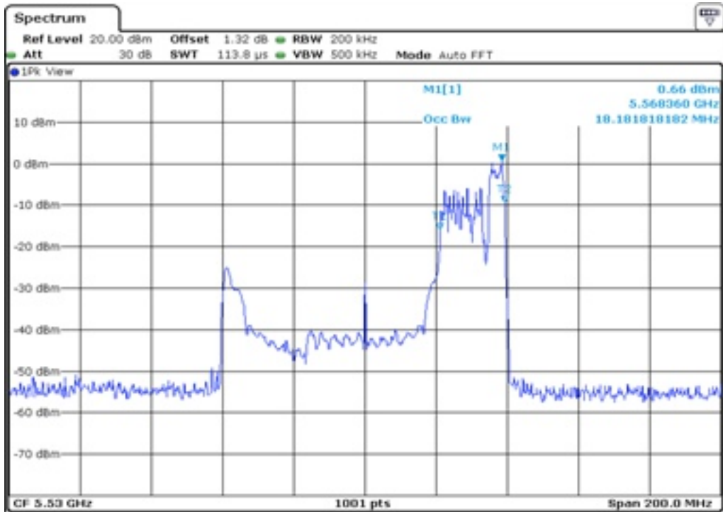
6 99% Occupied Bandwidth
