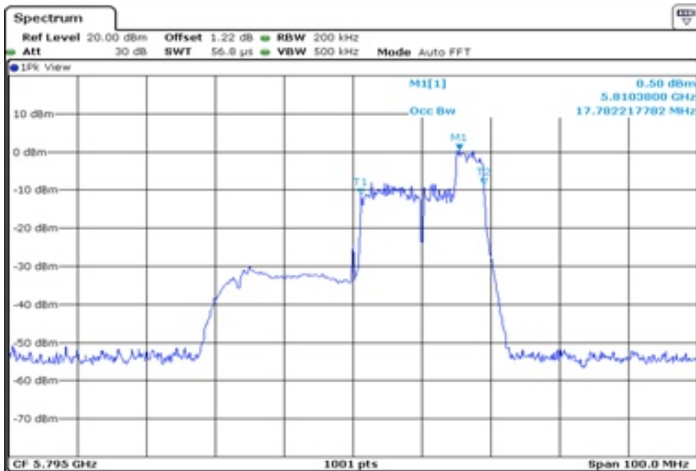
12 99% Occupied Bandwidth
