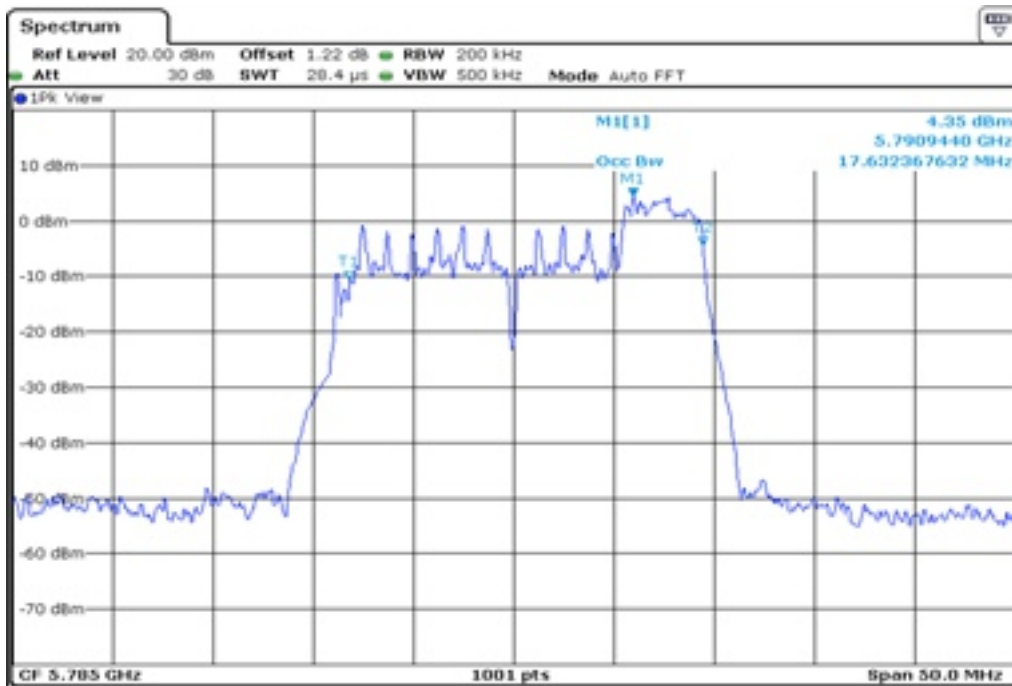
15 99% Occupied Bandwidth
