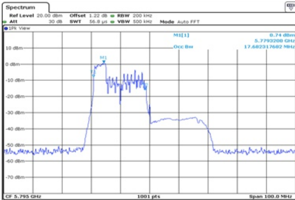
10 99% Occupied Bandwidth
