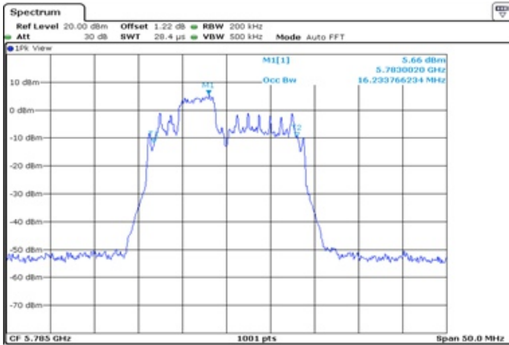
14 99% Occupied Bandwidth
