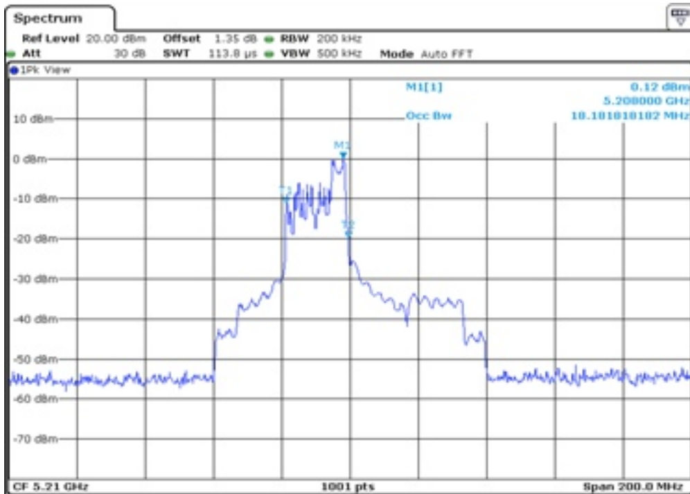
5 99% Occupied Bandwidth
