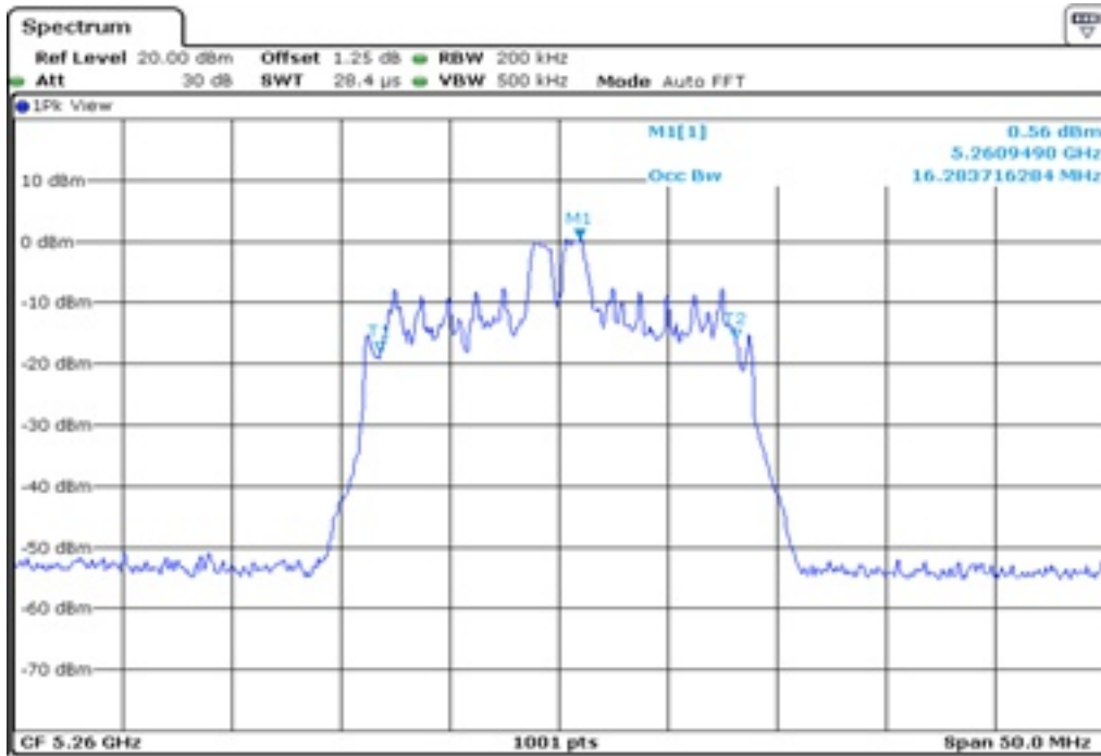
2 99% Occupied Bandwidth
