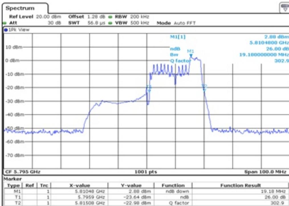
12 26 dB Bandwidth
