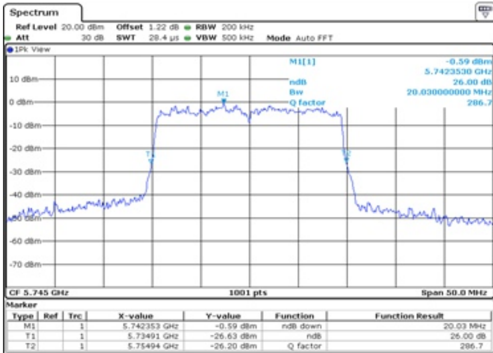
25 26 dB Bandwidth
