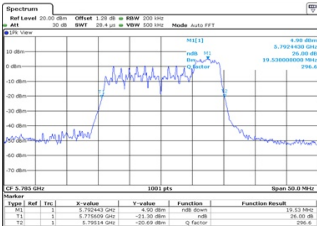
15 26 dB Bandwidth
