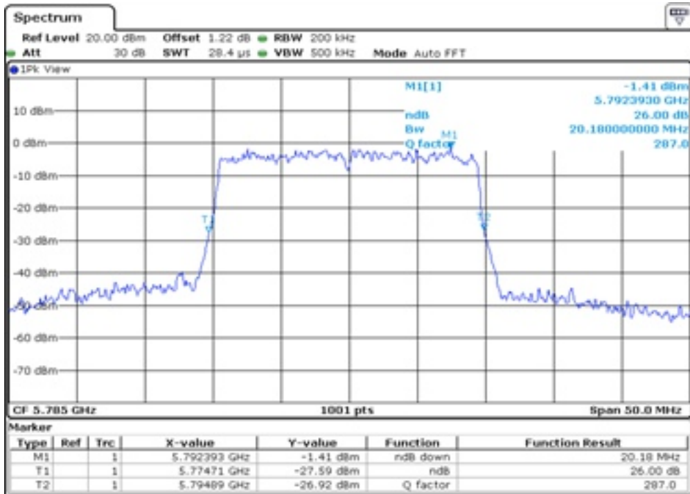
26 26 dB Bandwidth
