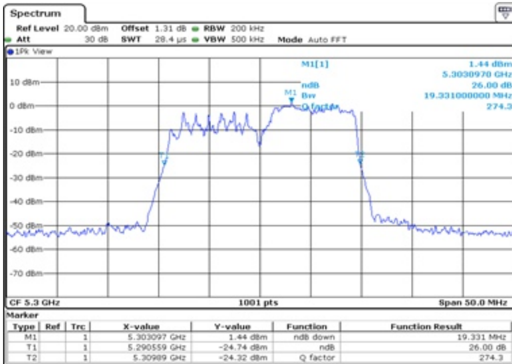
22 26 dB Bandwidth
