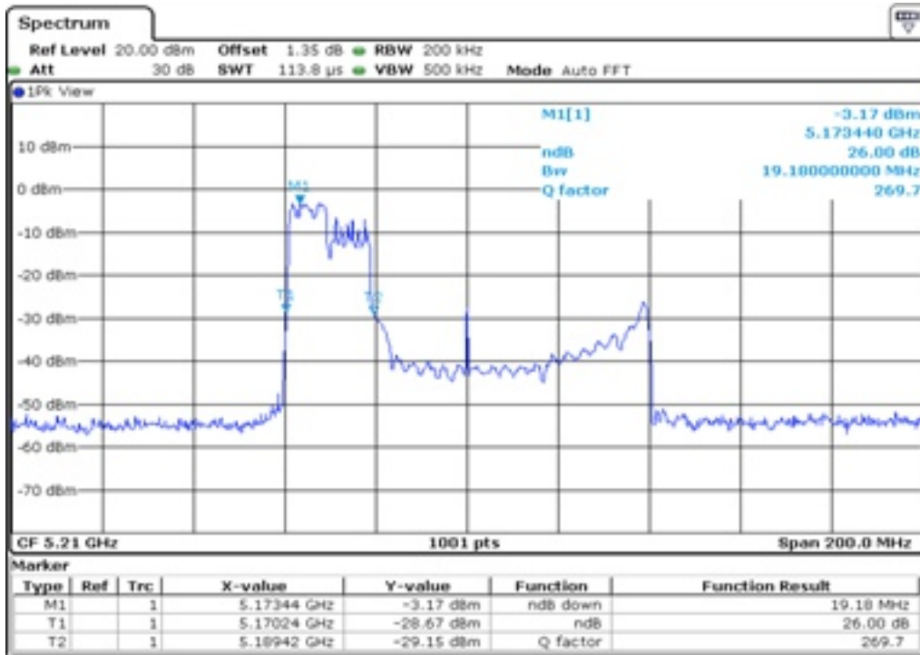
7 26 dB Bandwidth
