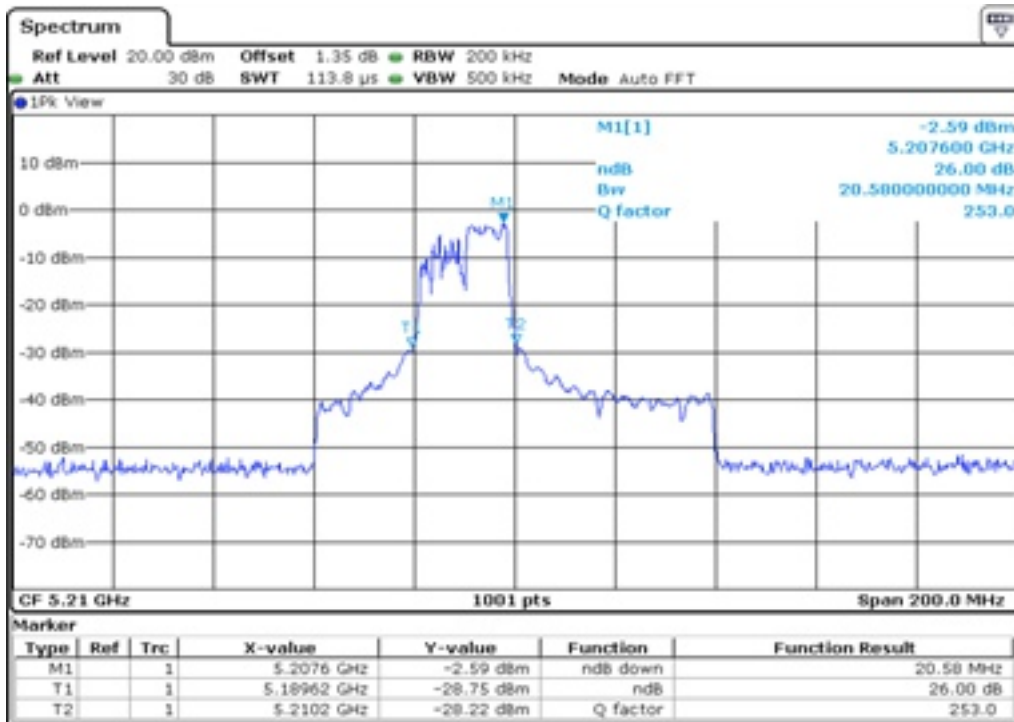
8 26 dB Bandwidth
