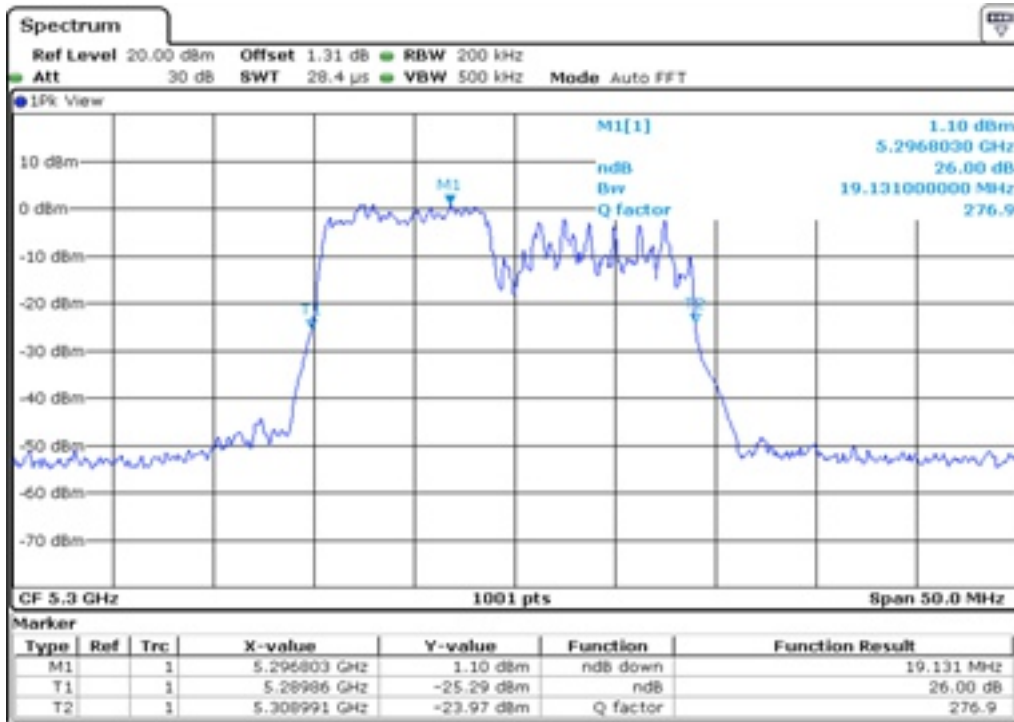
21 26 dB Bandwidth
