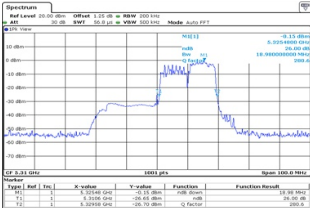
18 26 dB Bandwidth
