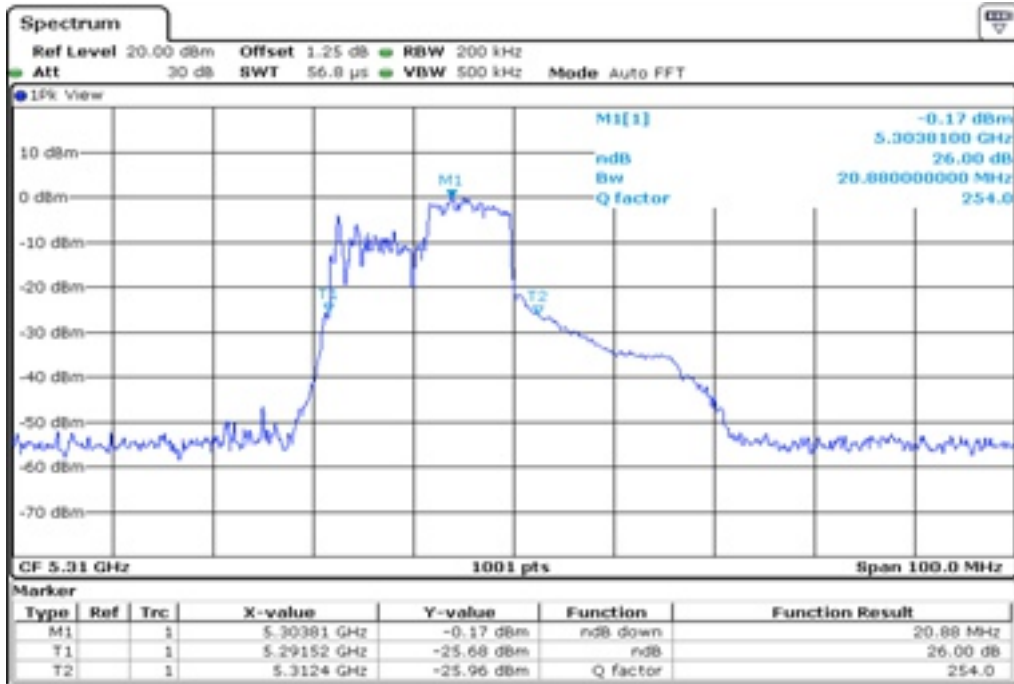
17 26 dB Bandwidth
