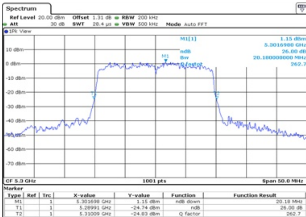
29 26 dB Bandwidth
