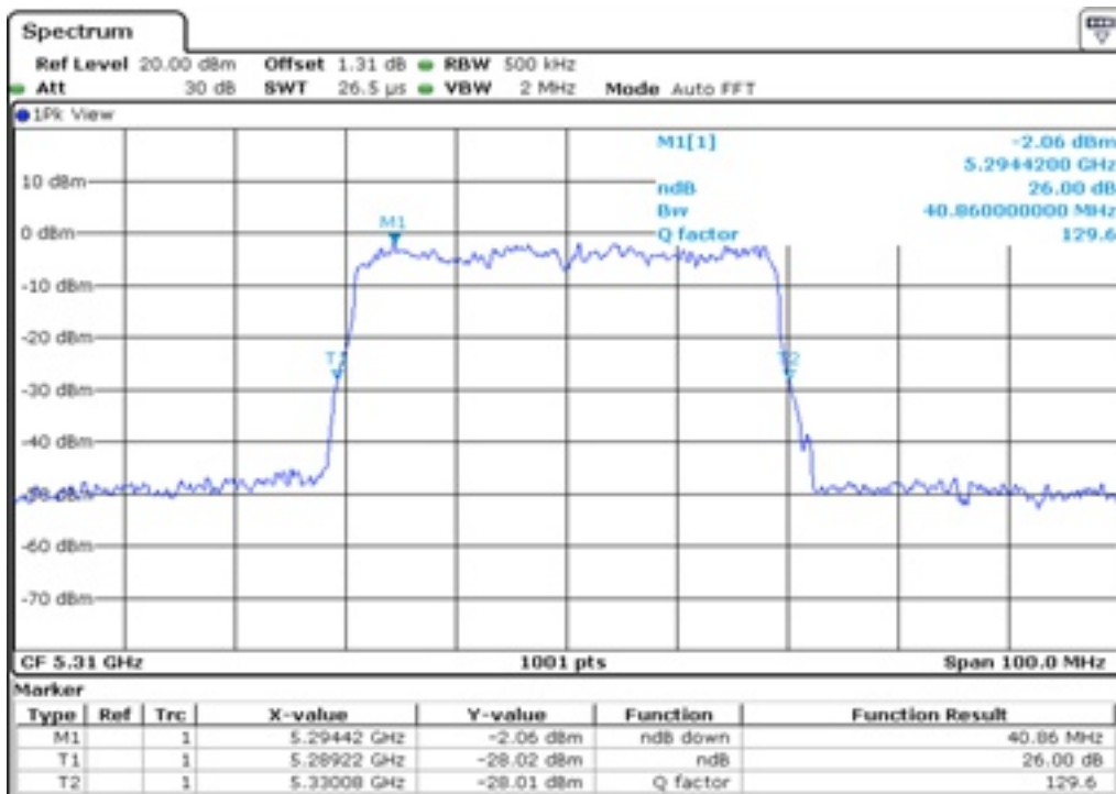
24 26 dB Bandwidth
