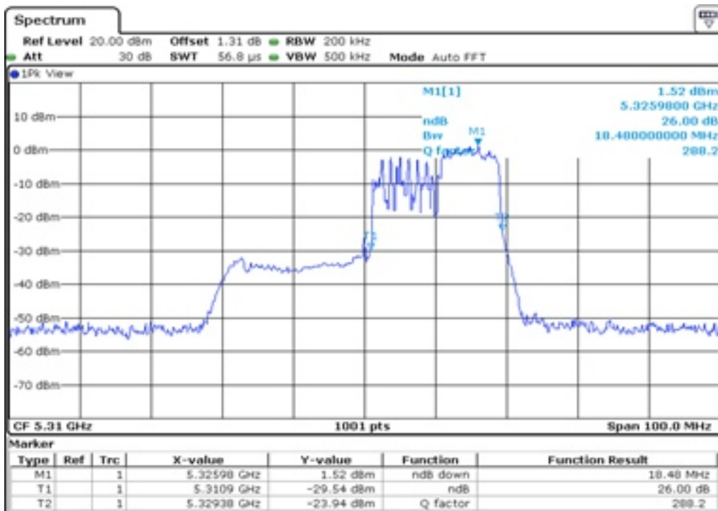
18 26 dB Bandwidth
