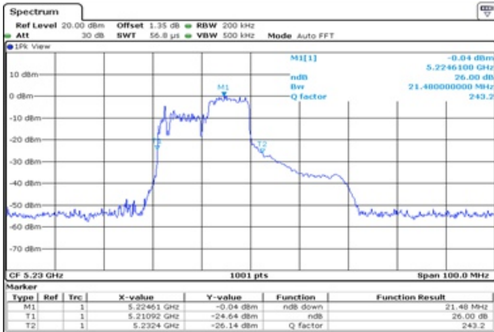
17 26 dB Bandwidth
