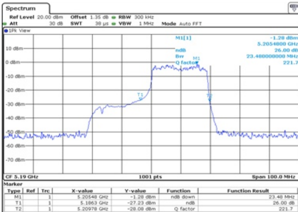
20 26 dB Bandwidth
