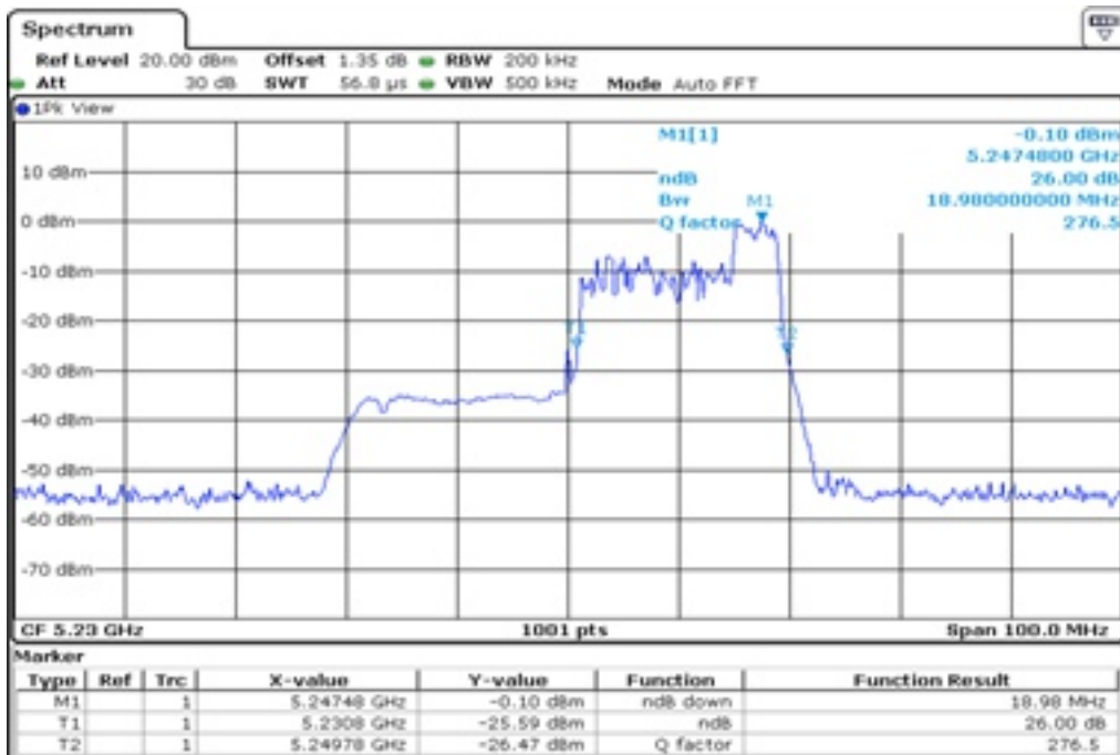
12 26 dB Bandwidth
