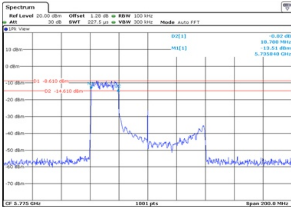
10 6 dB Bandwidth
