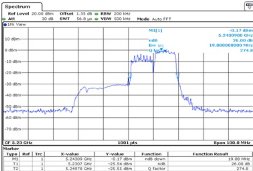
18 26 dB Bandwidth
