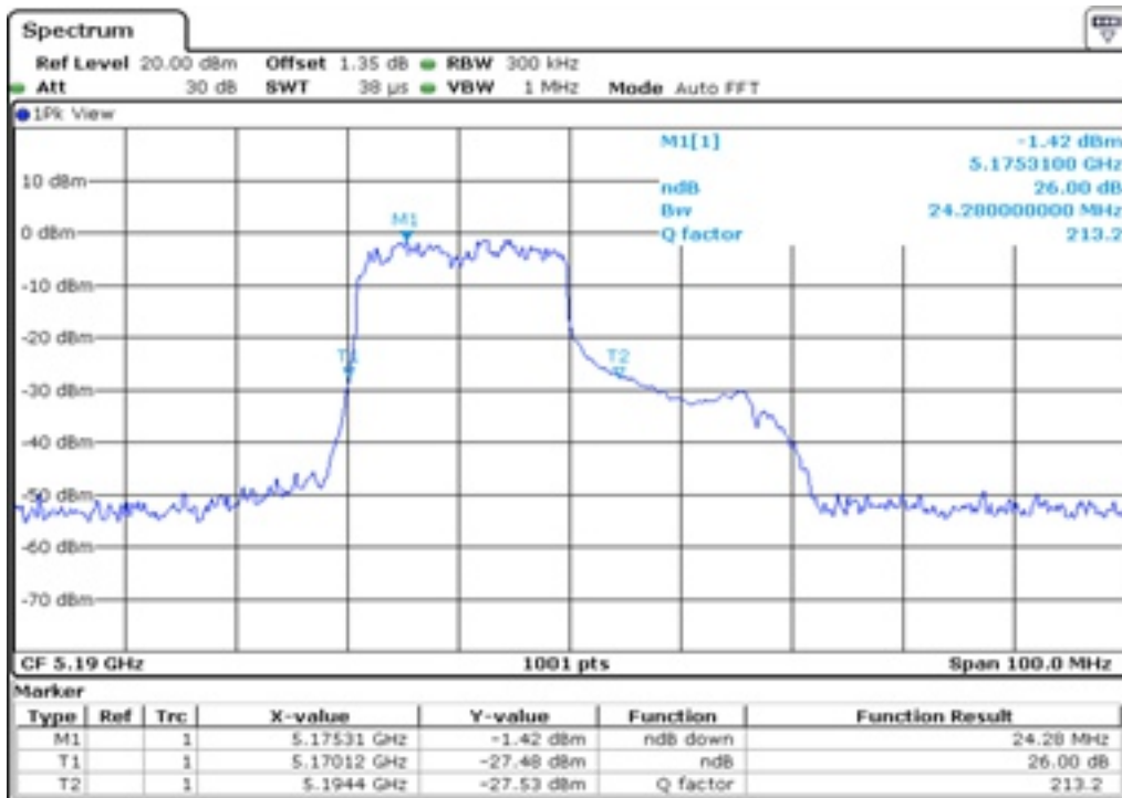
19 26 dB Bandwidth
