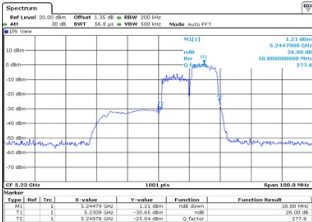
18 26 dB Bandwidth
