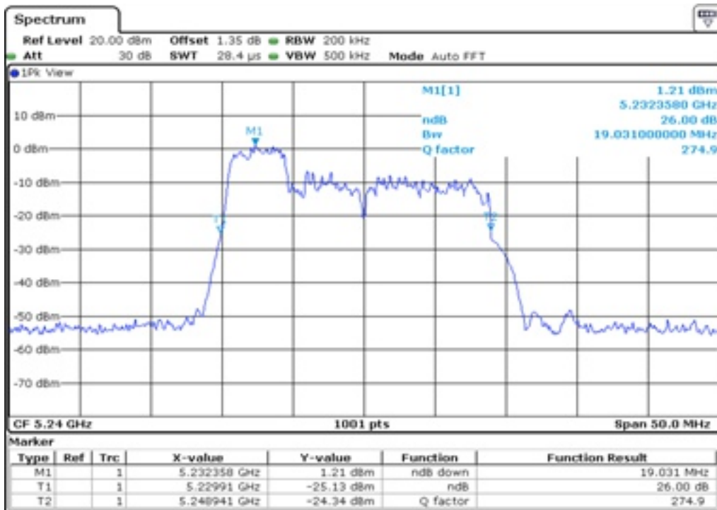
16 26 dB Bandwidth
