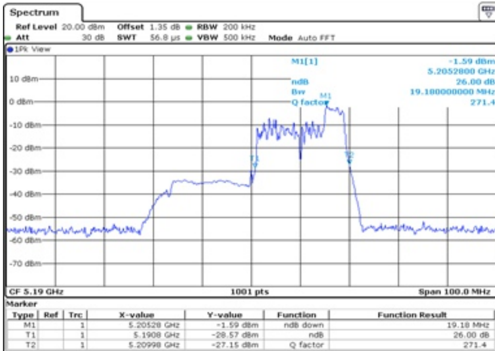
9 26 dB Bandwidth
