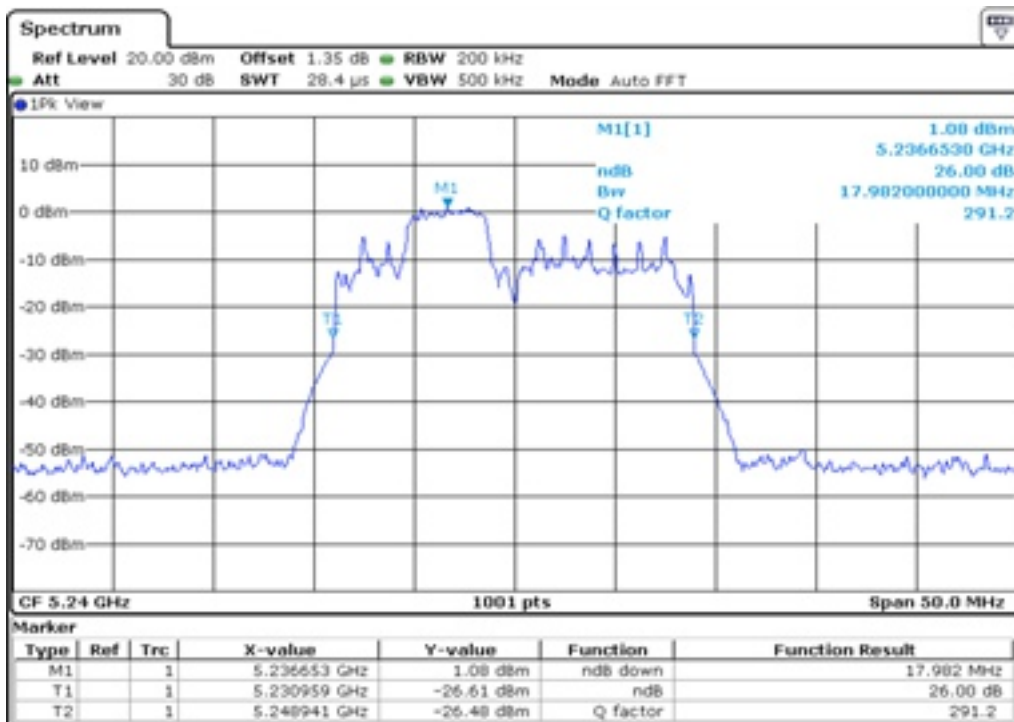
17 26 dB Bandwidth
