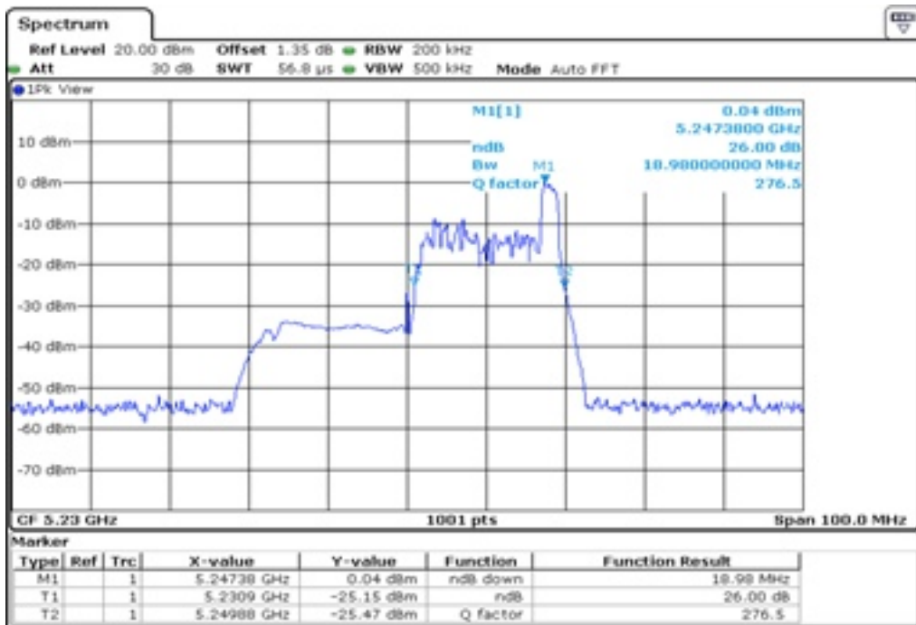
6 26 dB Bandwidth
