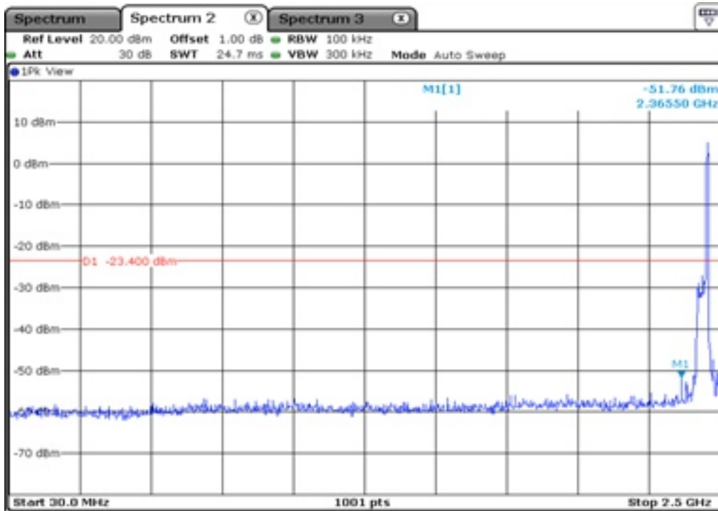
6.1 100 kHz Bandwidth
