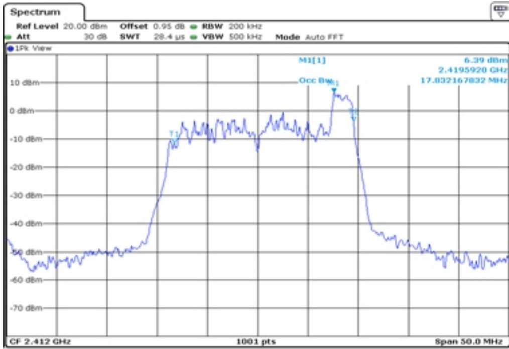
3 99% Occupied Bandwidth
