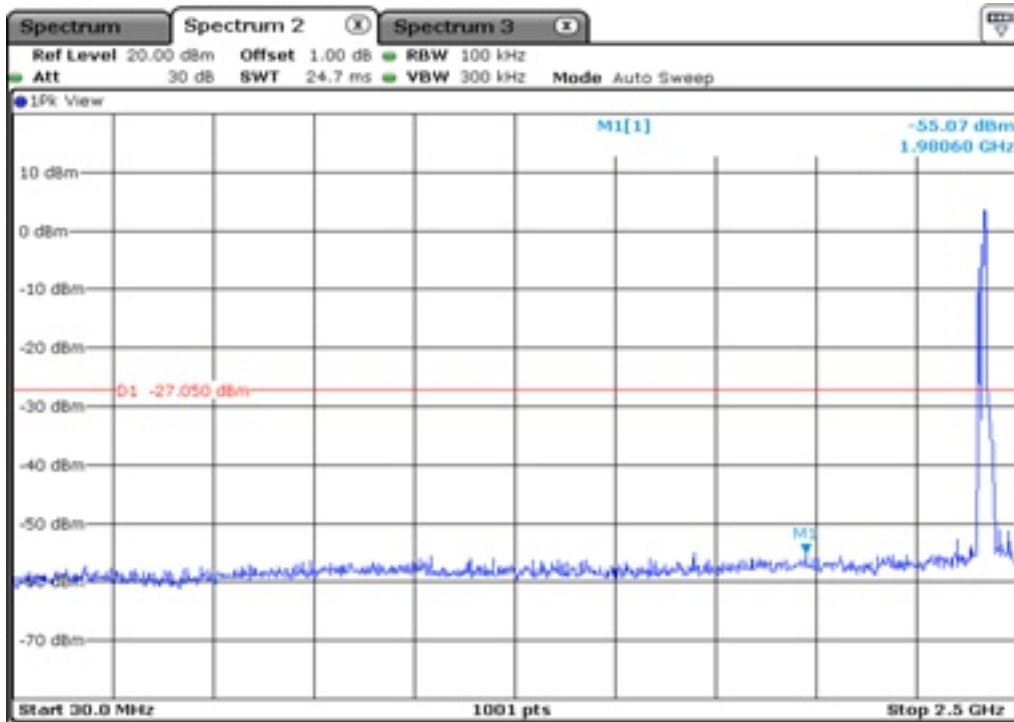
11.1 100 kHz Bandwidth
