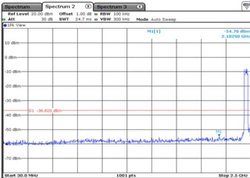
39.1 100 kHz Bandwidth
