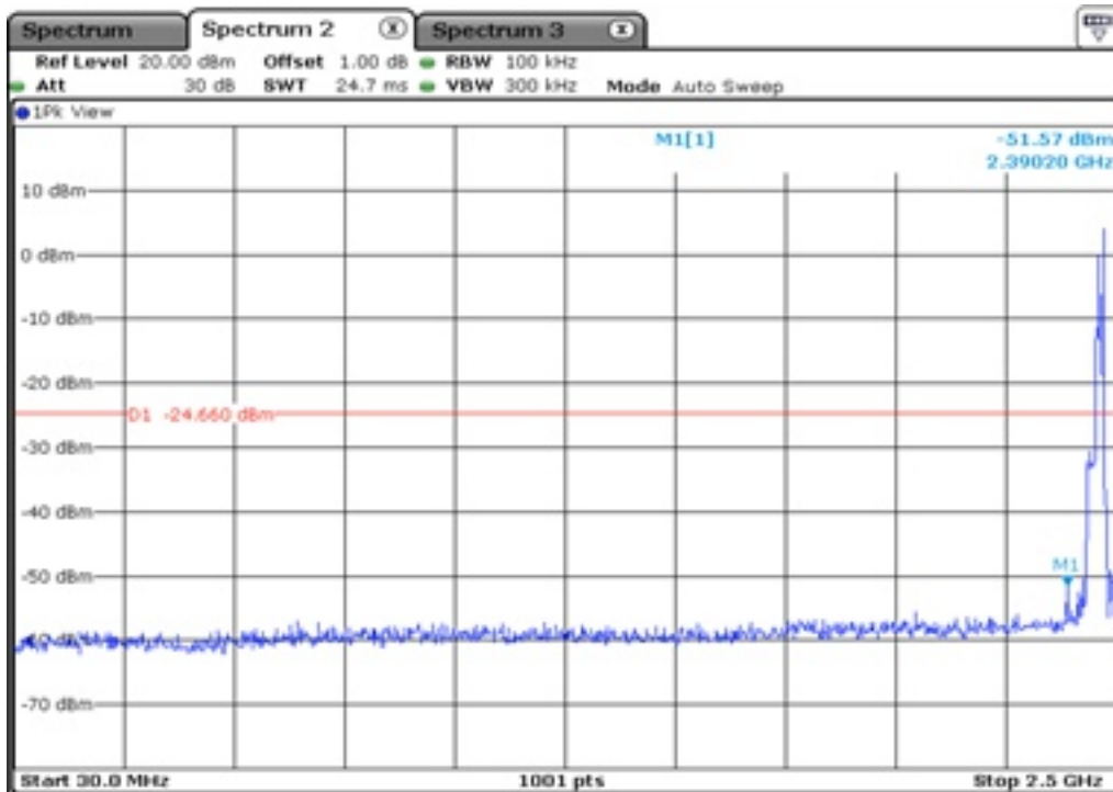
9.1 100 kHz Bandwidth
