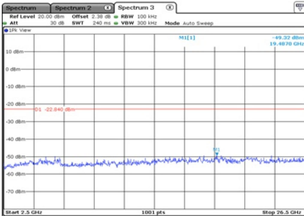
5.2 100 kHz Bandwidth
