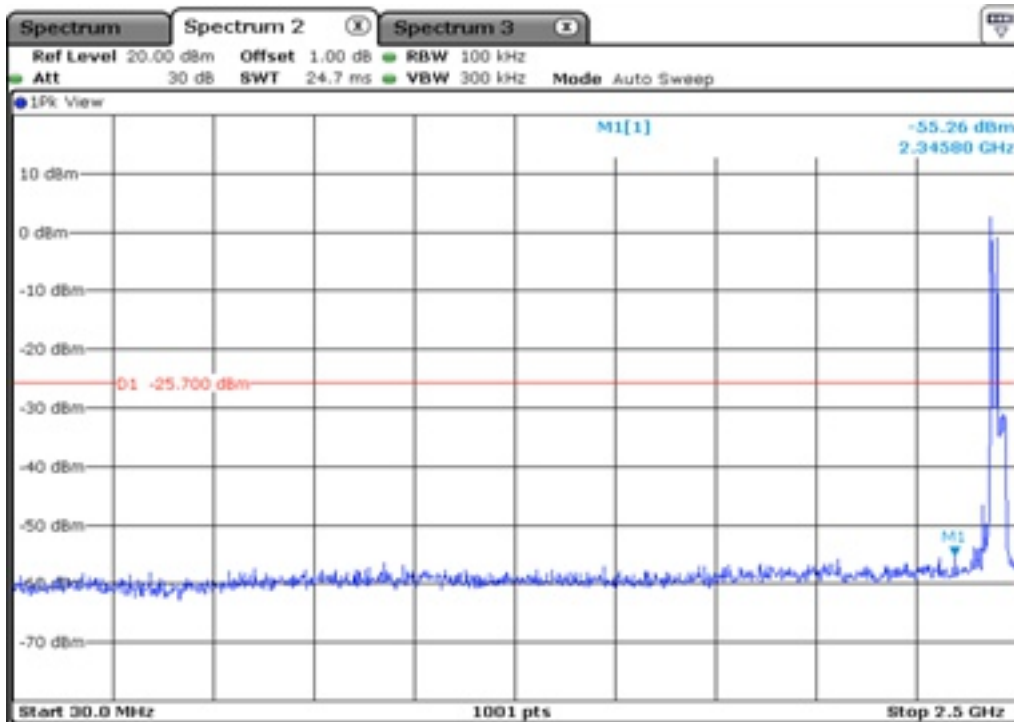
7.1 100 kHz Bandwidth
