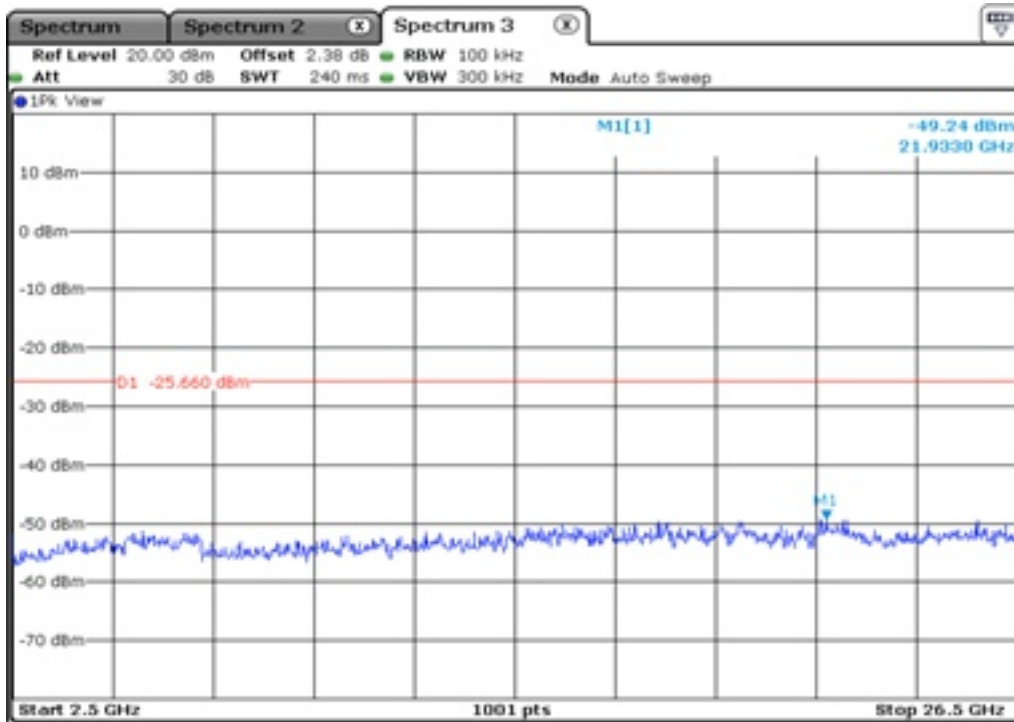
14.2 100 kHz Bandwidth
