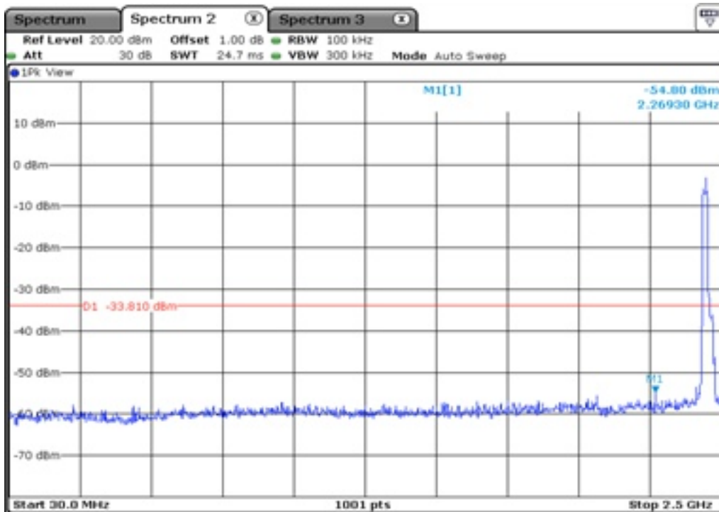
32.1 100 kHz Bandwidth
