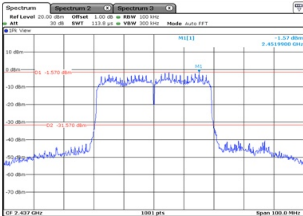
35 100 kHz Bandwidth
