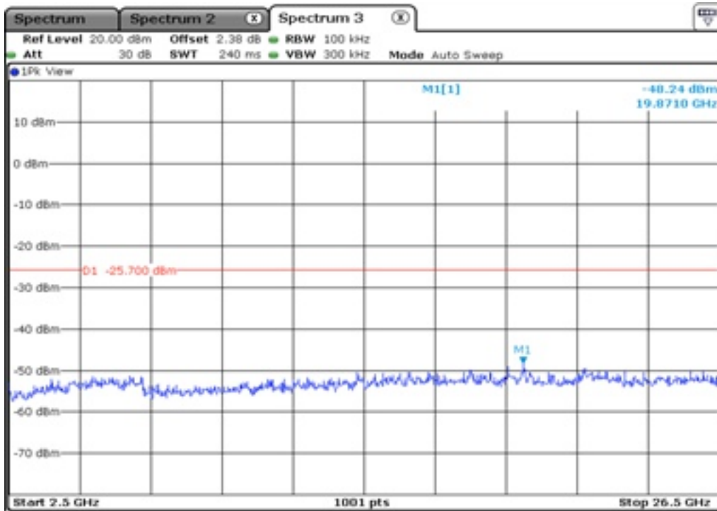
7.2 100 kHz Bandwidth
