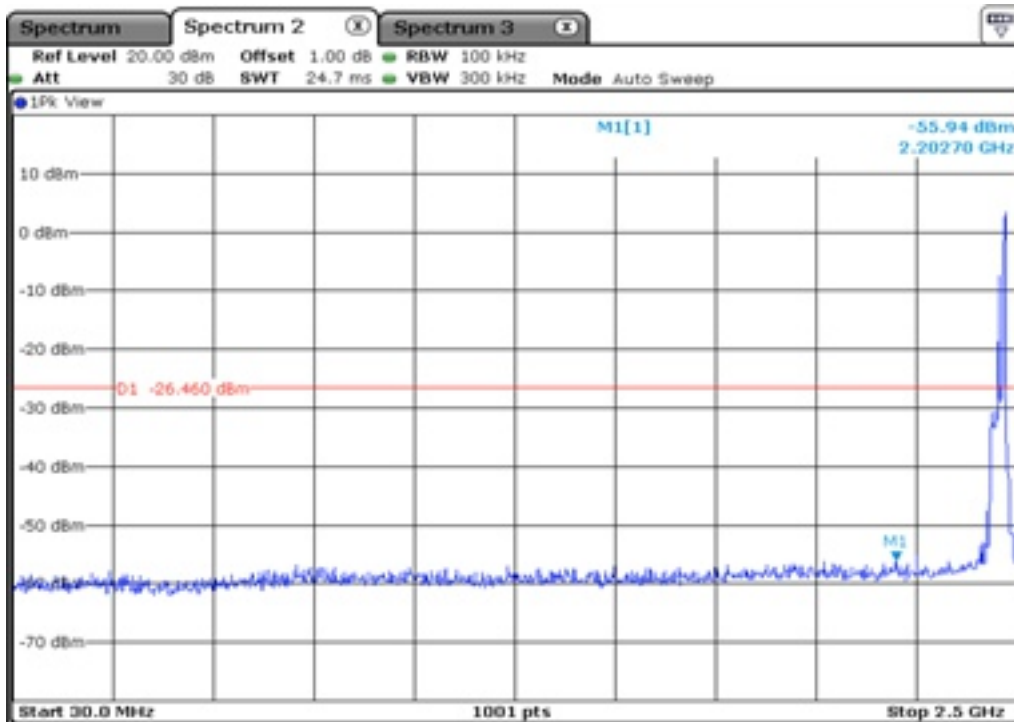
18.1 100 kHz Bandwidth
