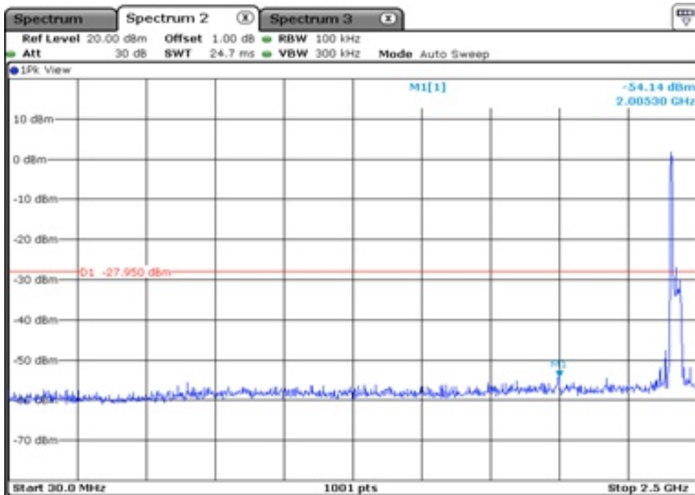
10.1 100 kHz Bandwidth
