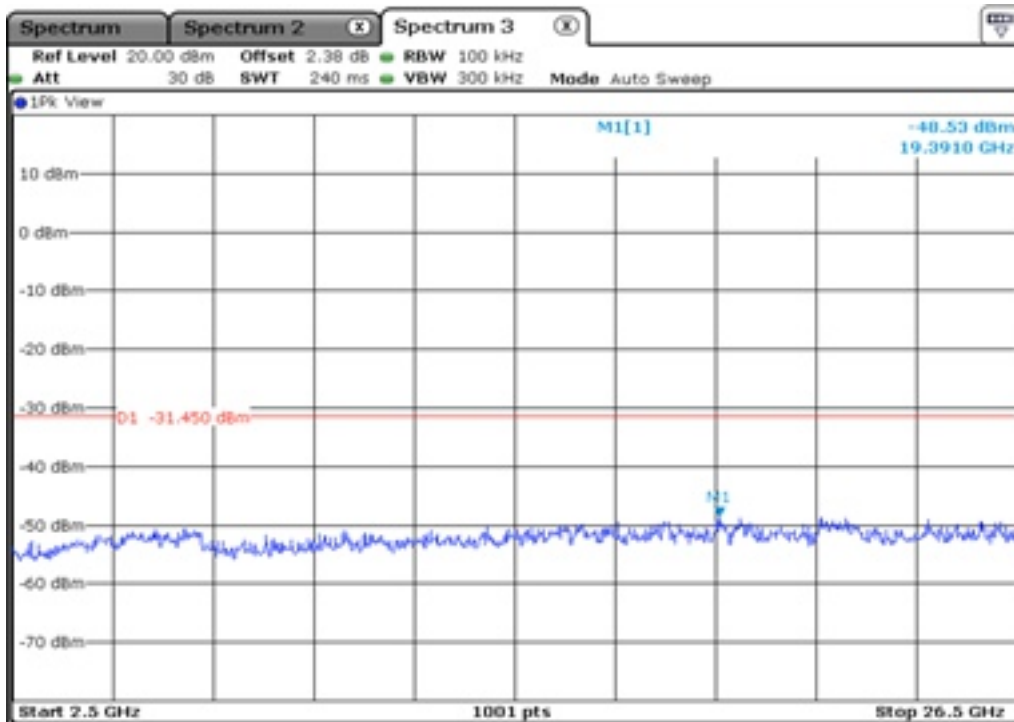
38.2 100 kHz Bandwidth
