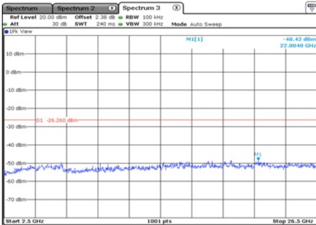
12.2 100 kHz Bandwidth
