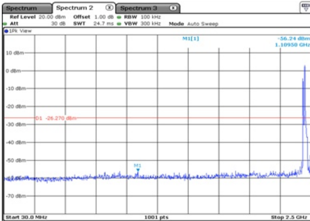
17.1 100 kHz Bandwidth
