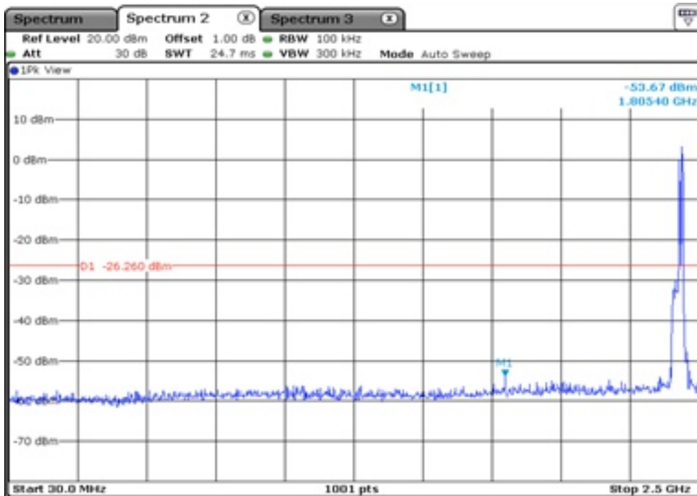
12.1 100 kHz Bandwidth
