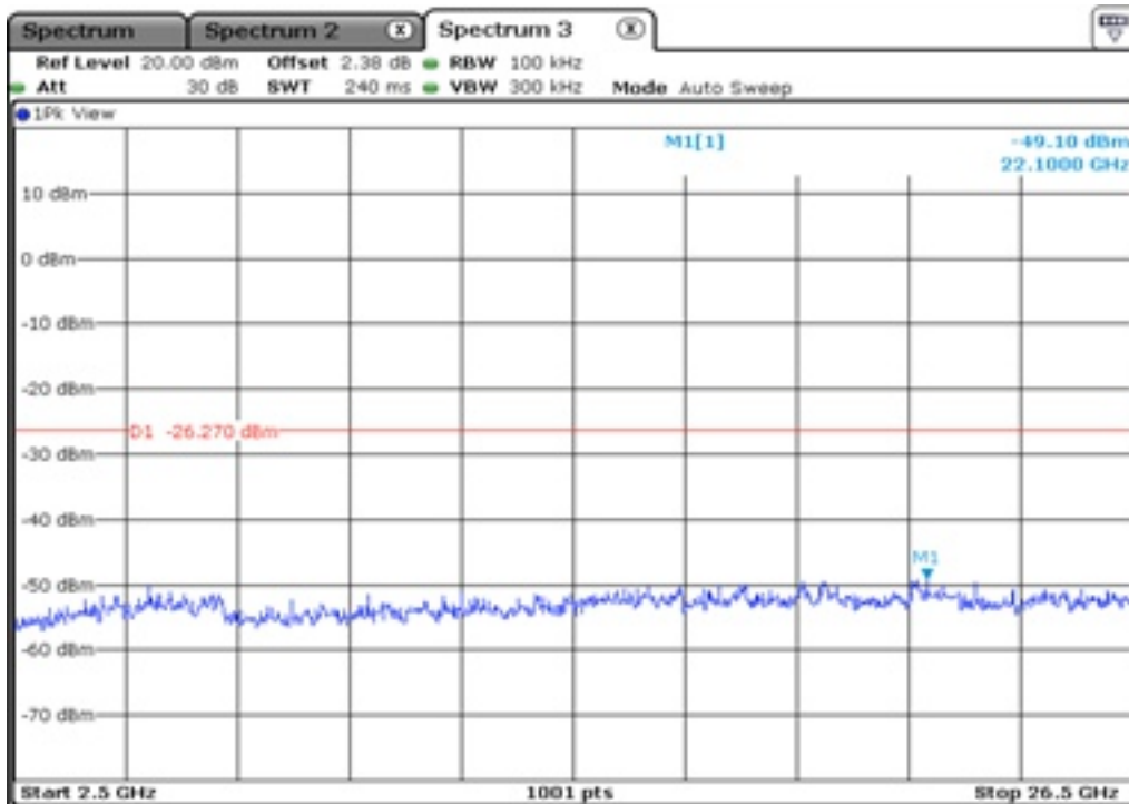
17.2 100 kHz Bandwidth
