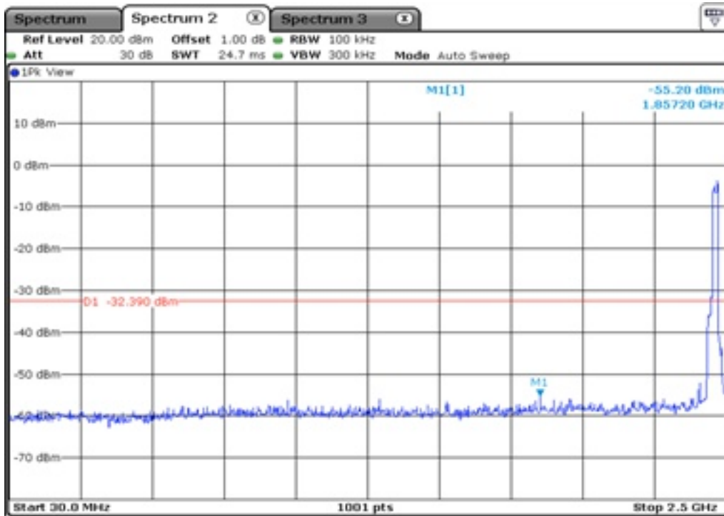
33.1 100 kHz Bandwidth
