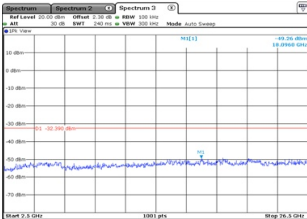
33.2 100 kHz Bandwidth
