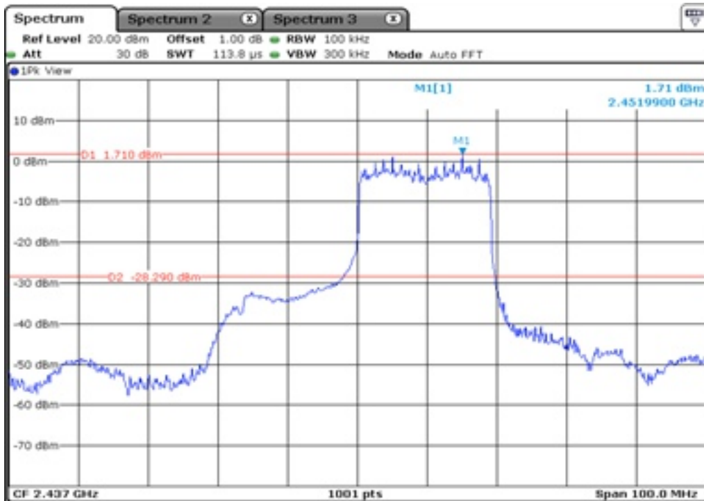
31 100 kHz Bandwidth
