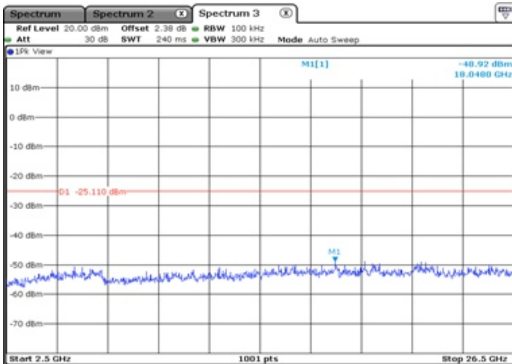
8.2 100 kHz Bandwidth
