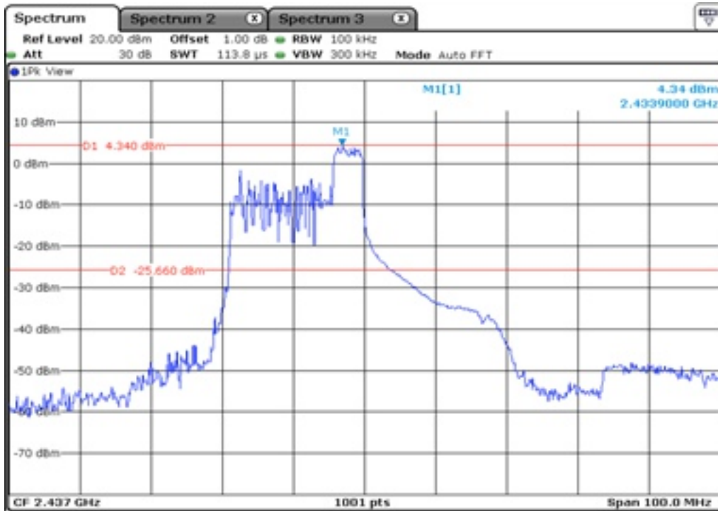
14 100 kHz Bandwidth
