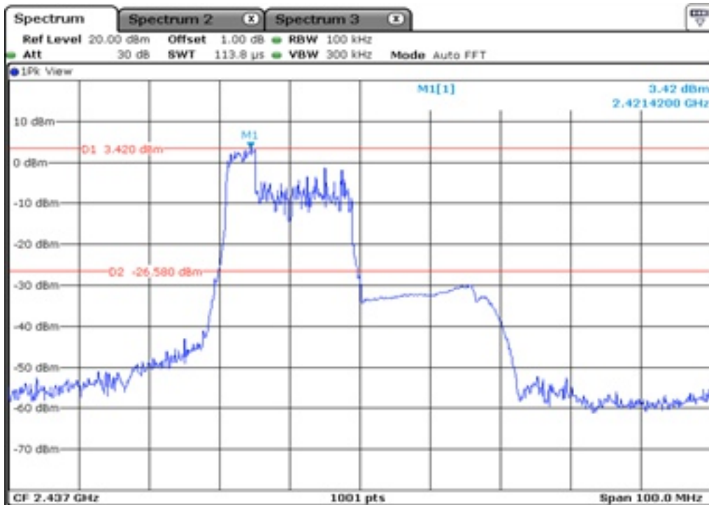
13 100 kHz Bandwidth
