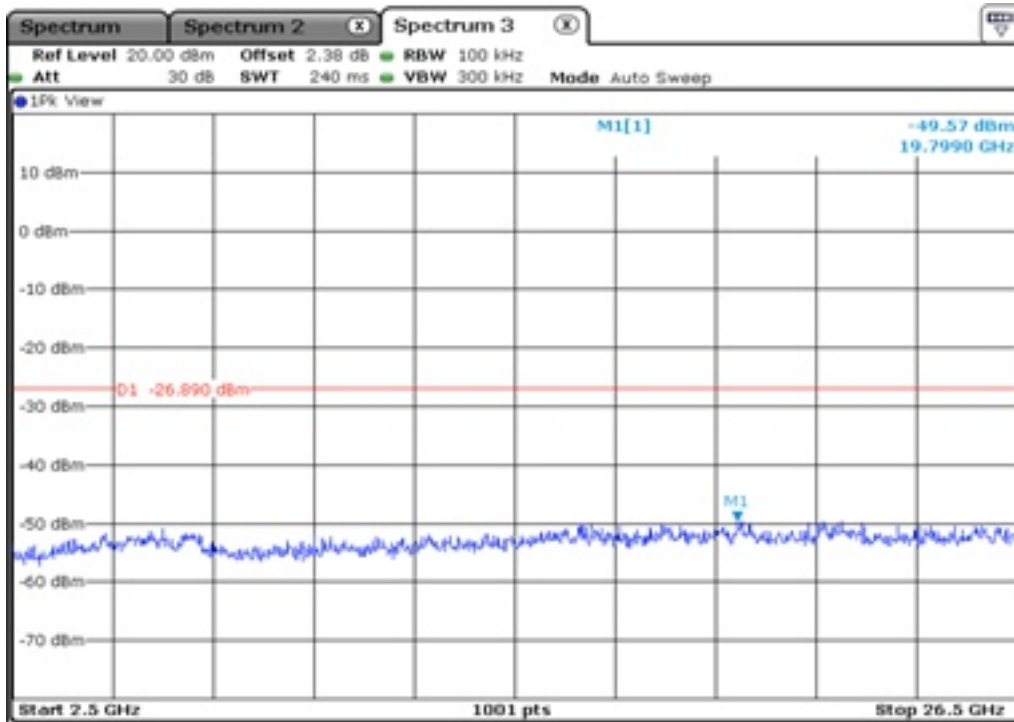
16.2 100 kHz Bandwidth
