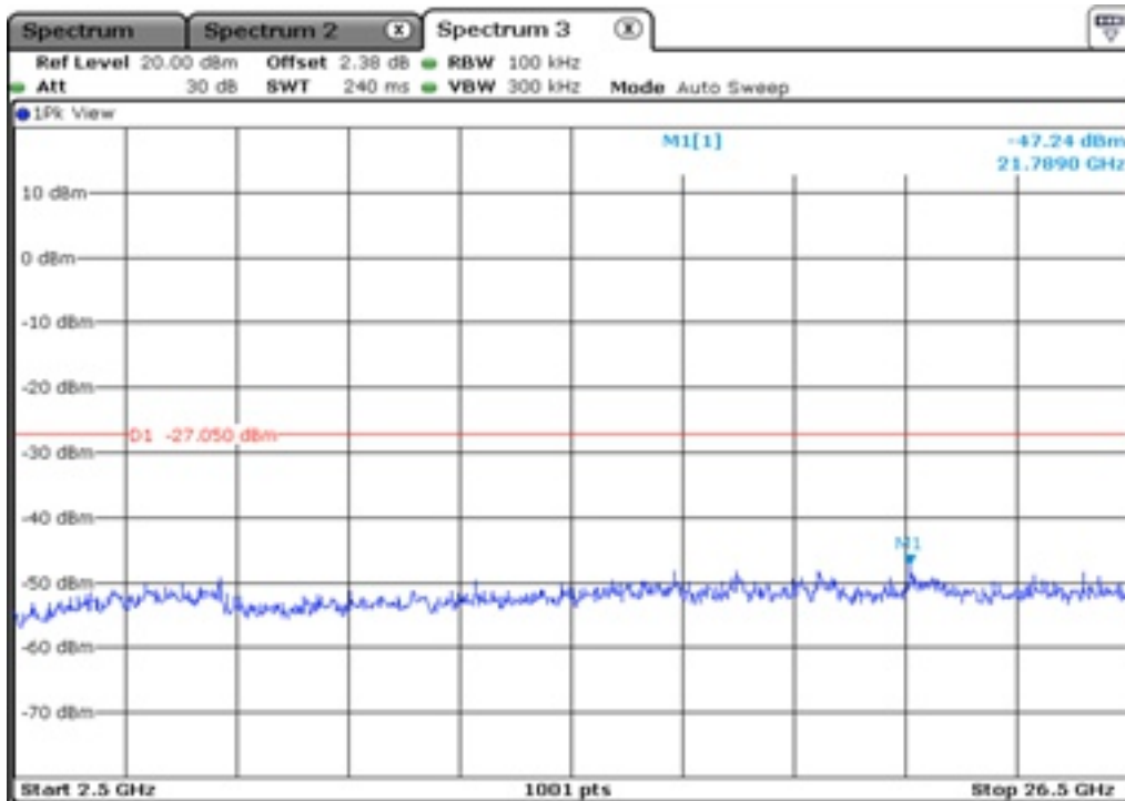
11.2 100 kHz Bandwidth
