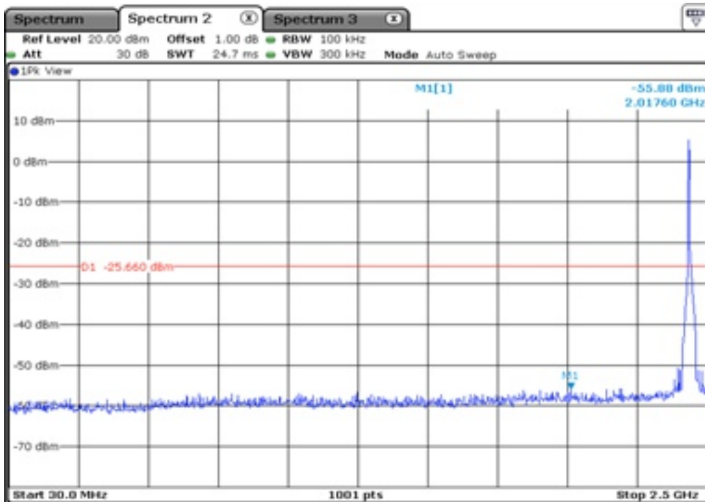
14.1 100 kHz Bandwidth
