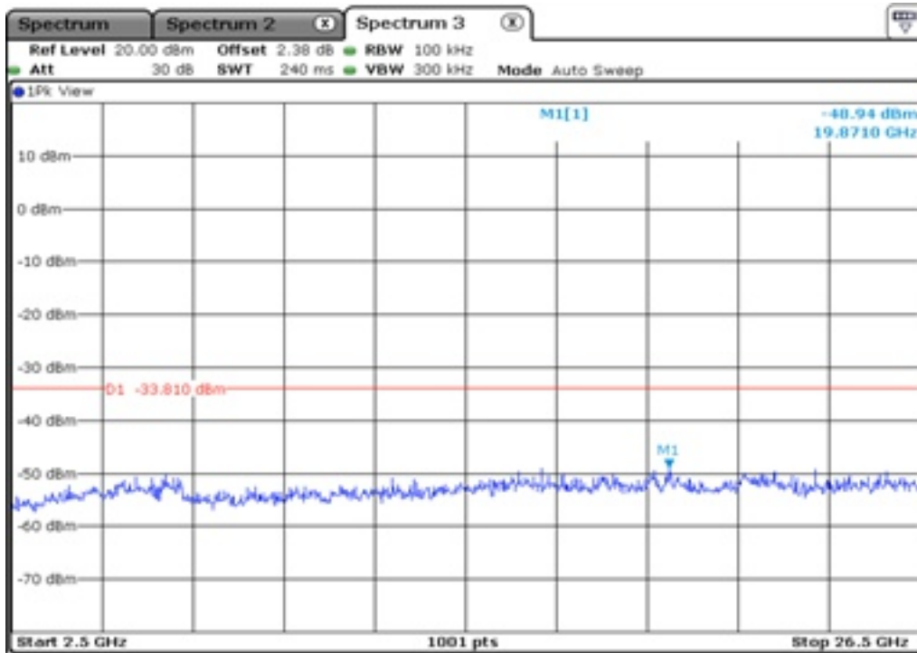
32.2 100 kHz Bandwidth
