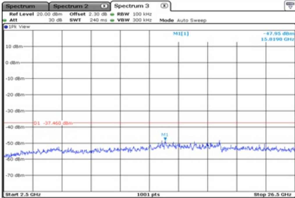
39.2 100 kHz Bandwidth
