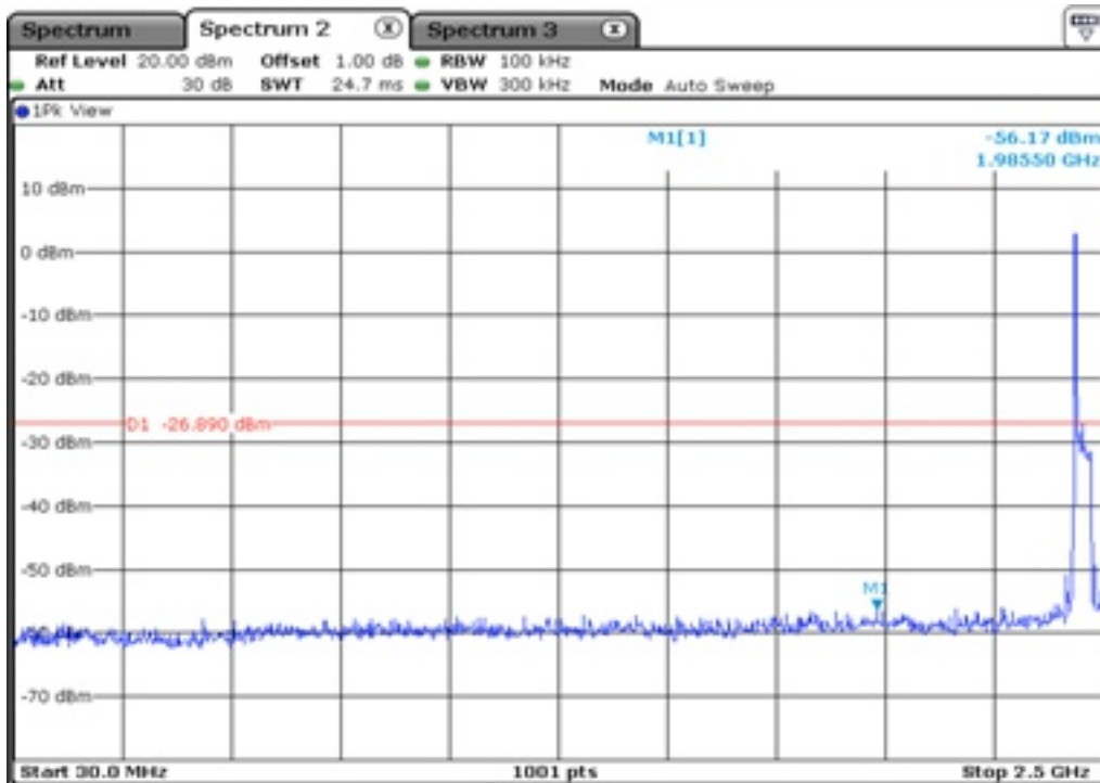
16.1 100 kHz Bandwidth
