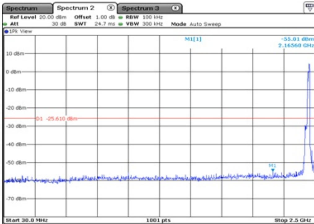
15.1 100 kHz Bandwidth
