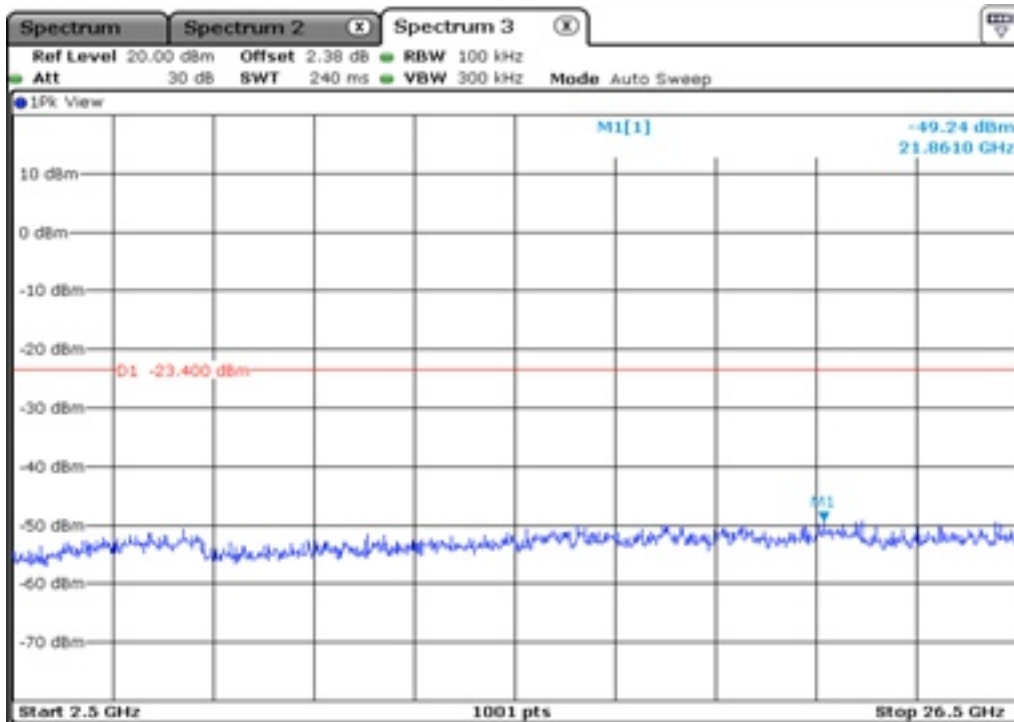
6.2 100 kHz Bandwidth
