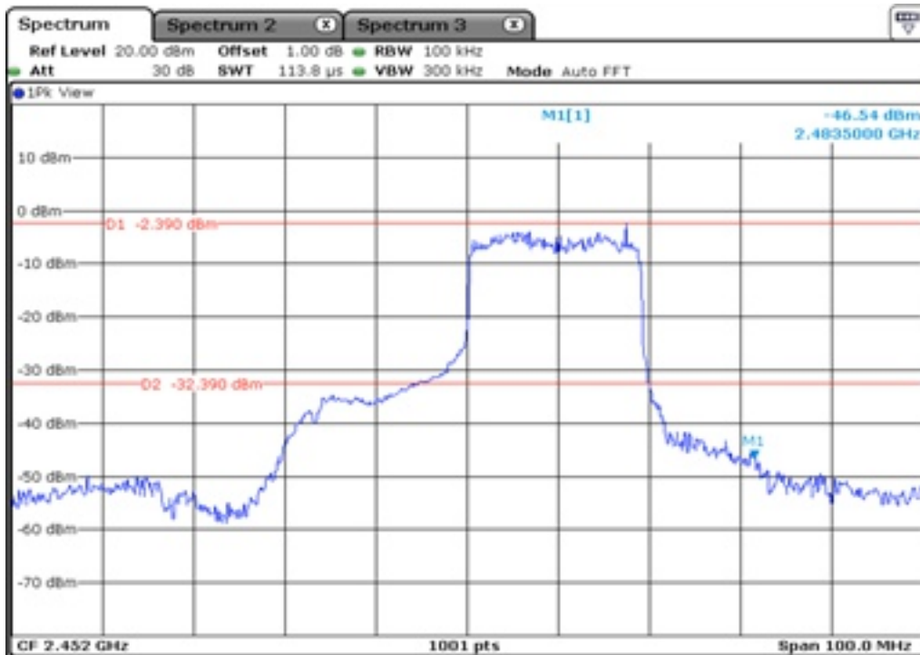
33 100 kHz Bandwidth
