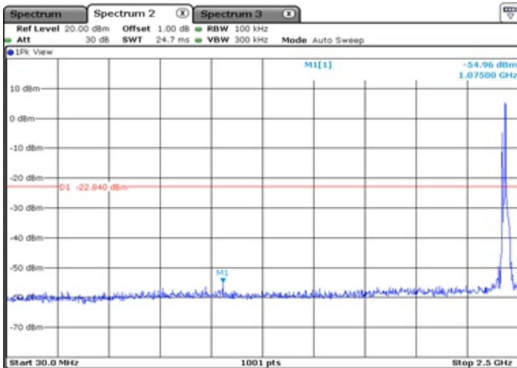
5.1 100 kHz Bandwidth
