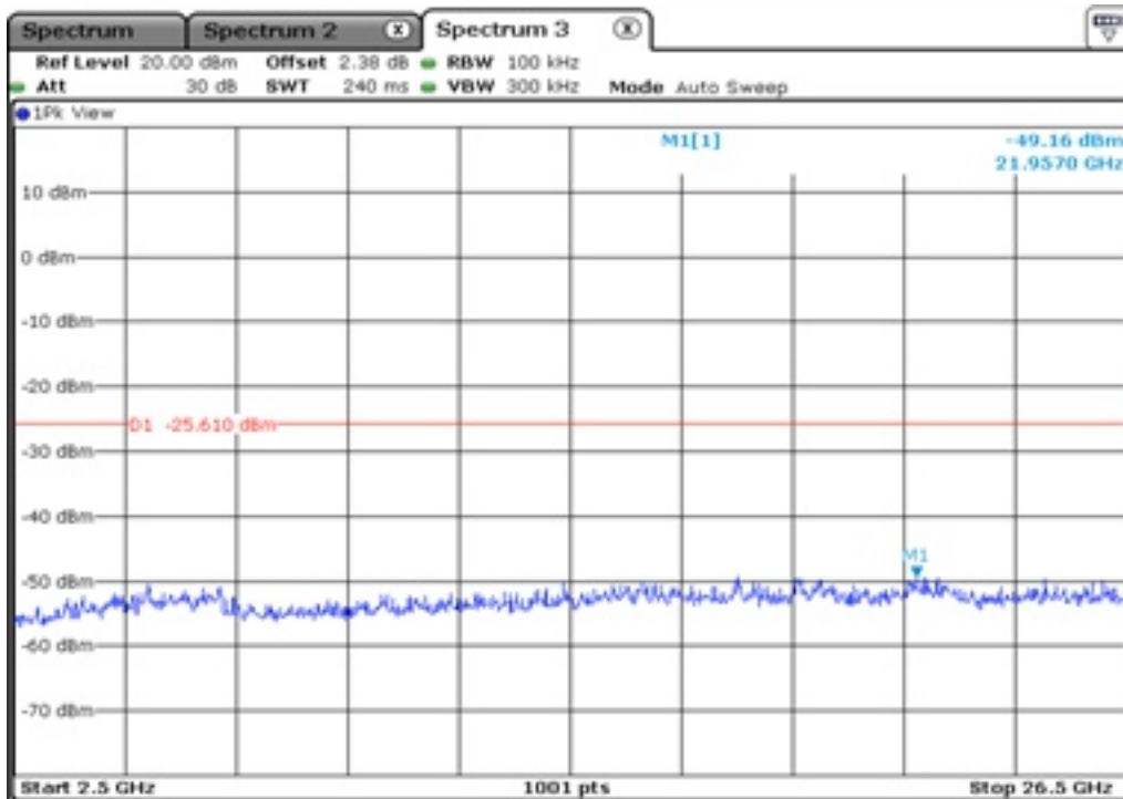
15.2 100 kHz Bandwidth
