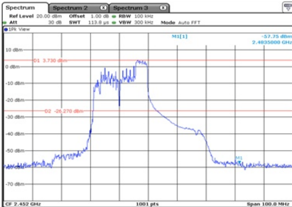
17 100 kHz Bandwidth
