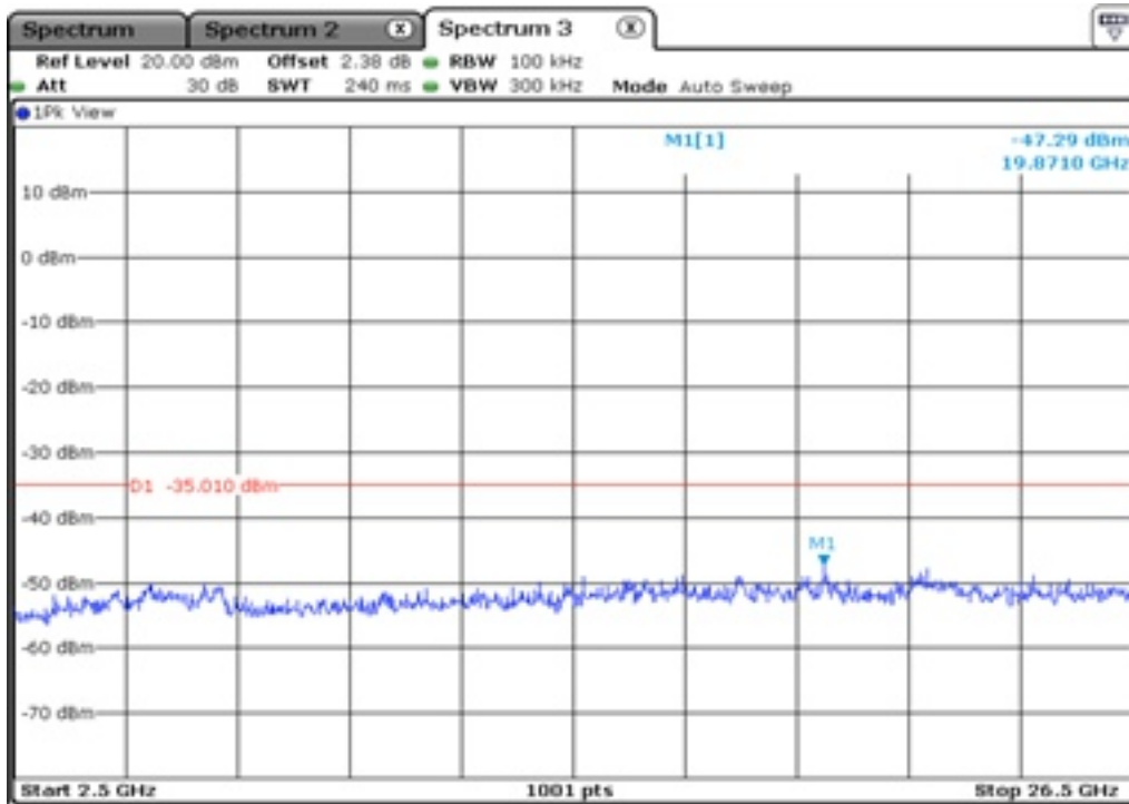
34.2 100 kHz Bandwidth
