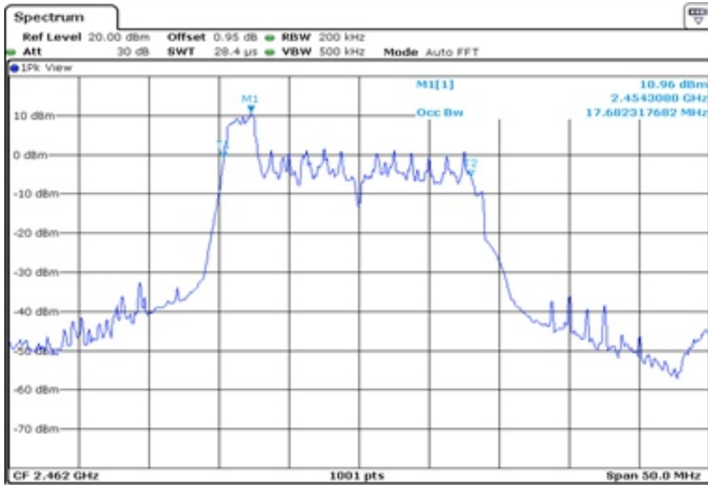
7 99% Occupied Bandwidth
