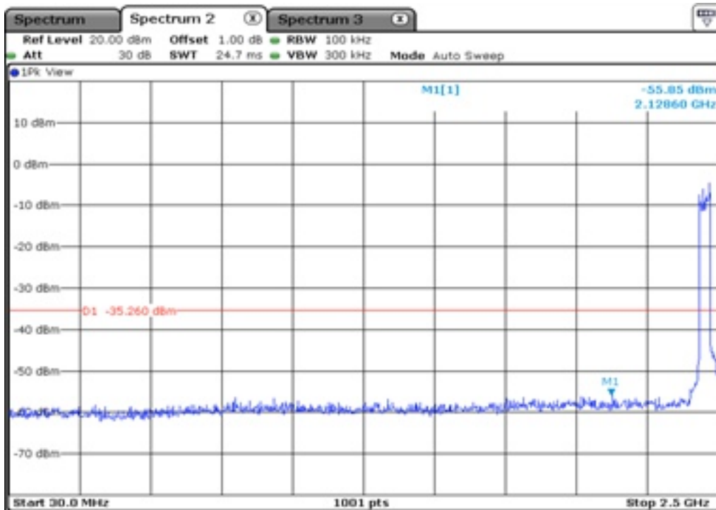
36.1 100 kHz Bandwidth
