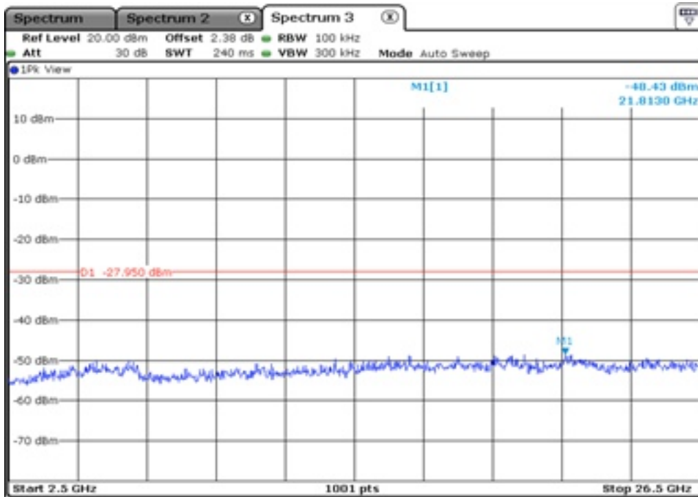
10.2 100 kHz Bandwidth
