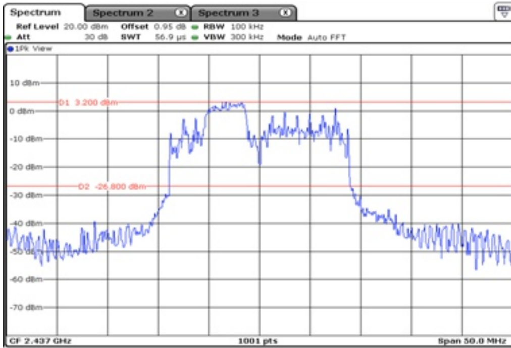
14 100 kHz Bandwidth
