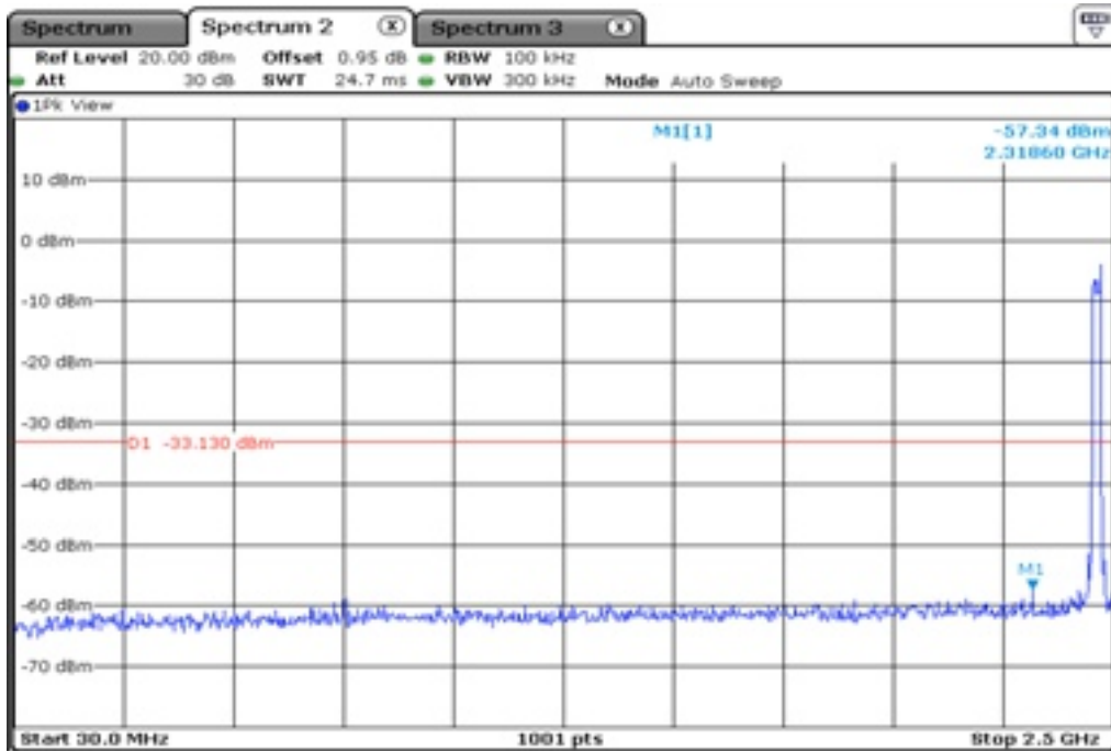
27.1 100 kHz Bandwidth
