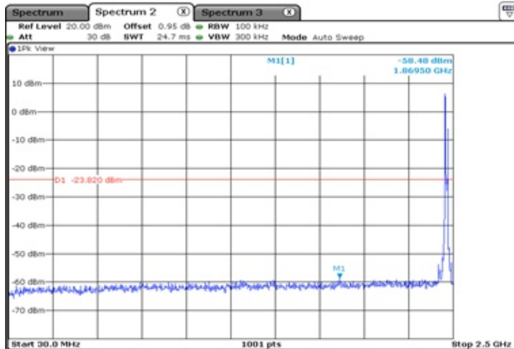
7.1 100 kHz Bandwidth
