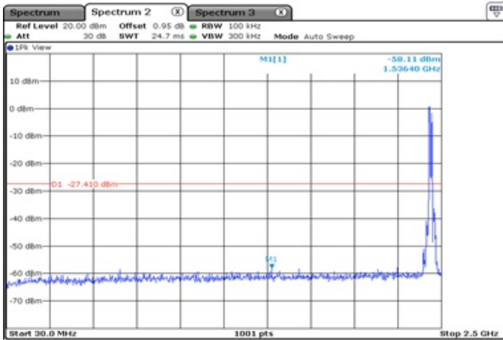
13.1 100 kHz Bandwidth
