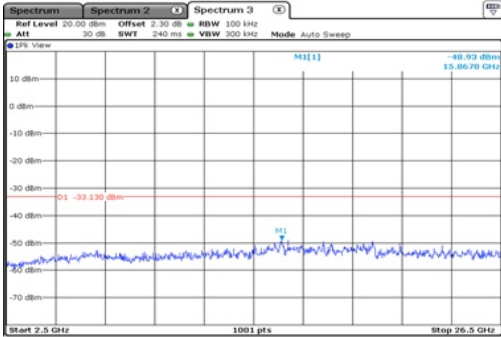
27.2 100 kHz Bandwidth
