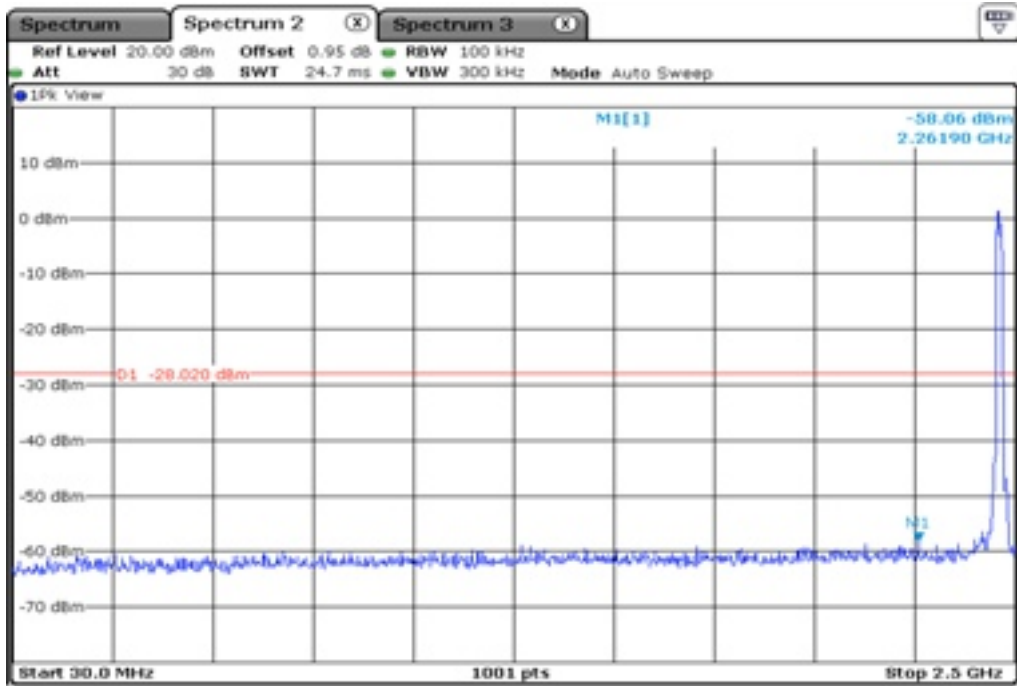
23.1 100 kHz Bandwidth
