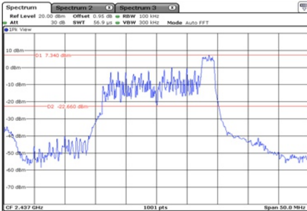
6 100 kHz Bandwidth
