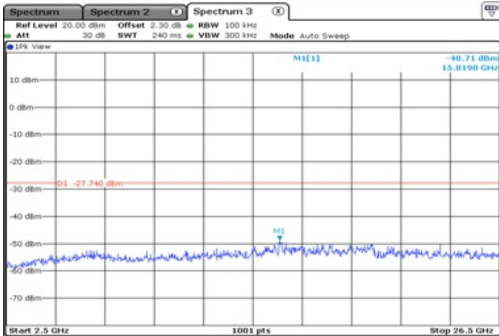
11.2 100 kHz Bandwidth
