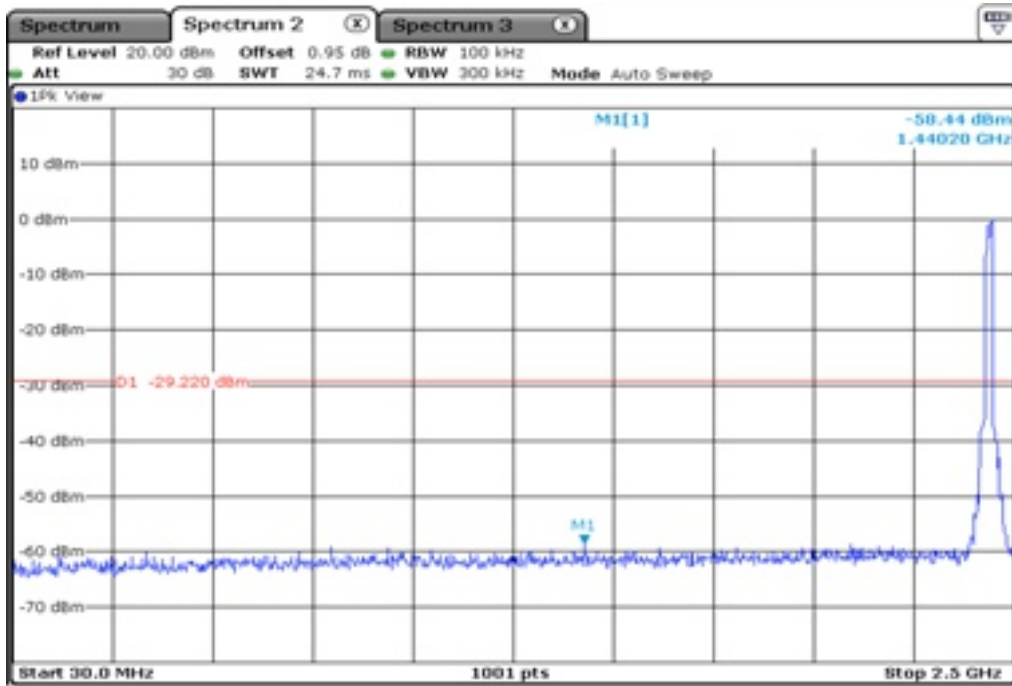
29.1 100 kHz Bandwidth
