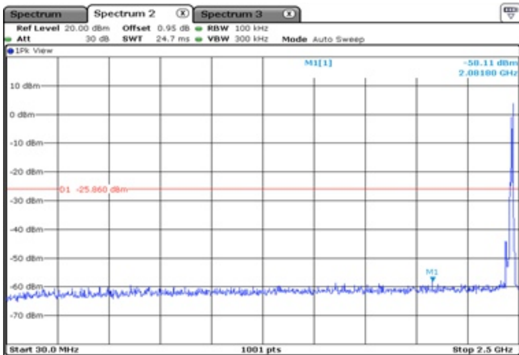
9.1 100 kHz Bandwidth
