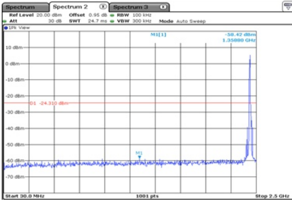
5.1 100 kHz Bandwidth
