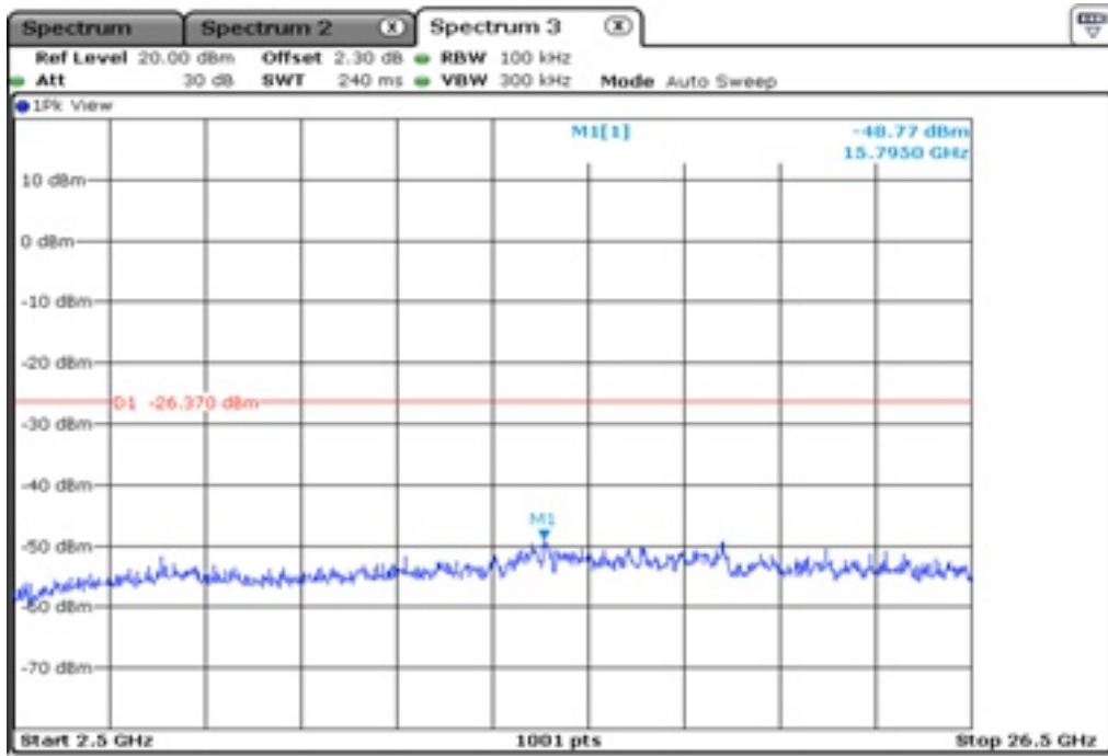
18.2 100 kHz Bandwidth
