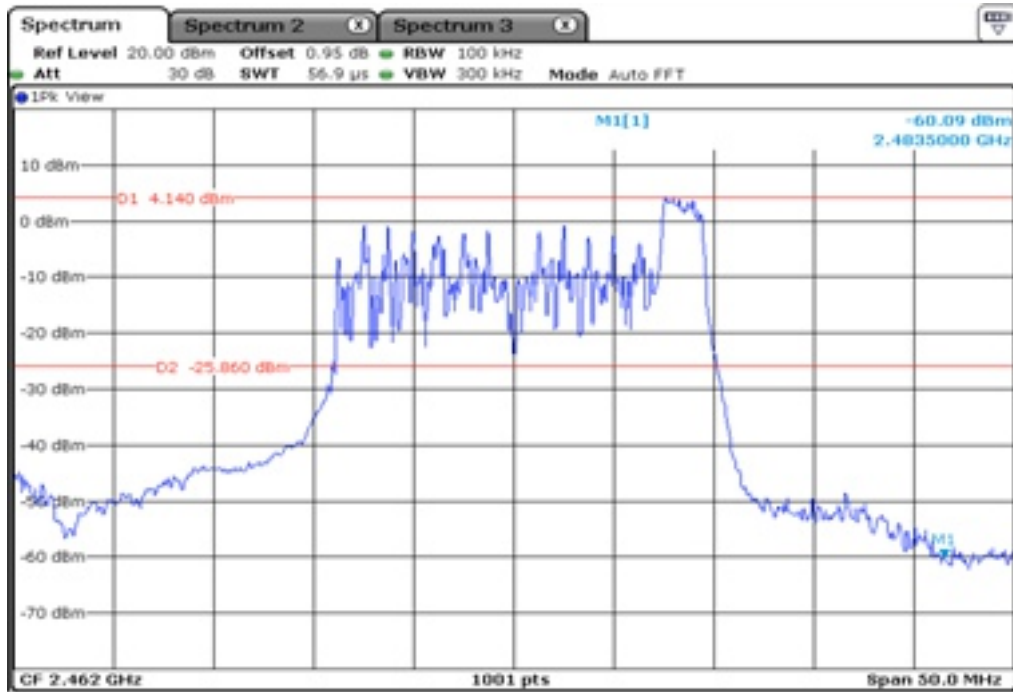
9 100 kHz Bandwidth
