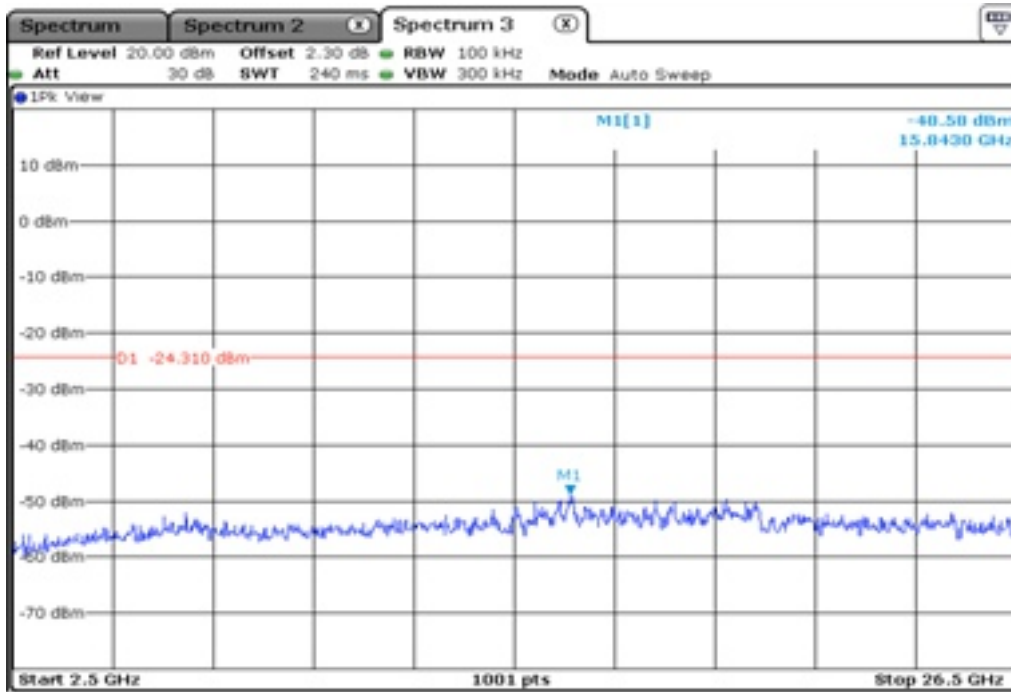
5.2 100 kHz Bandwidth
