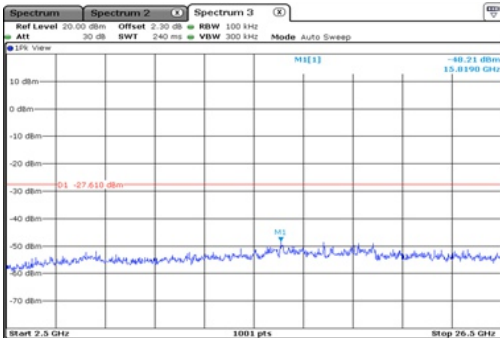
22.2 100 kHz Bandwidth
