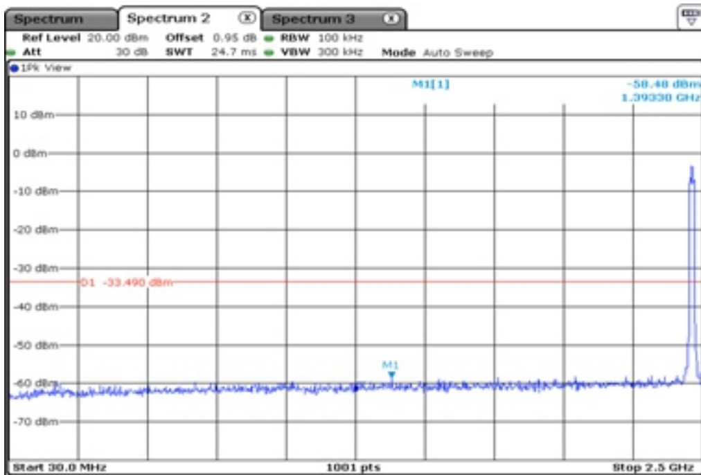
30.1 100 kHz Bandwidth
