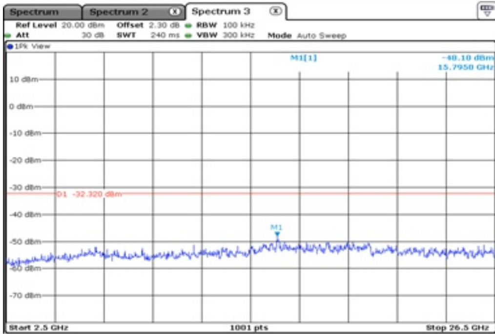
28.2 100 kHz Bandwidth
