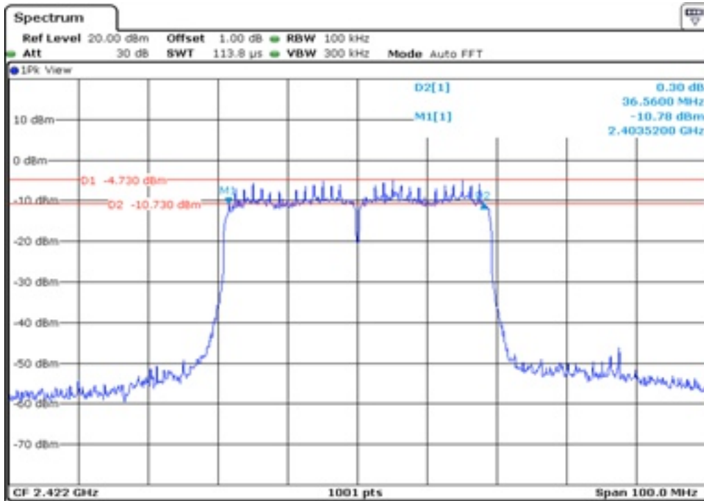
37 6 dB Bandwidth
