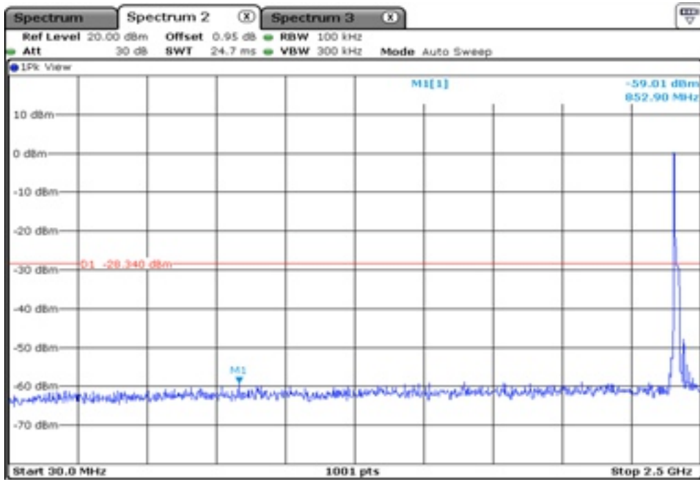
1.1 100 kHz Bandwidth
