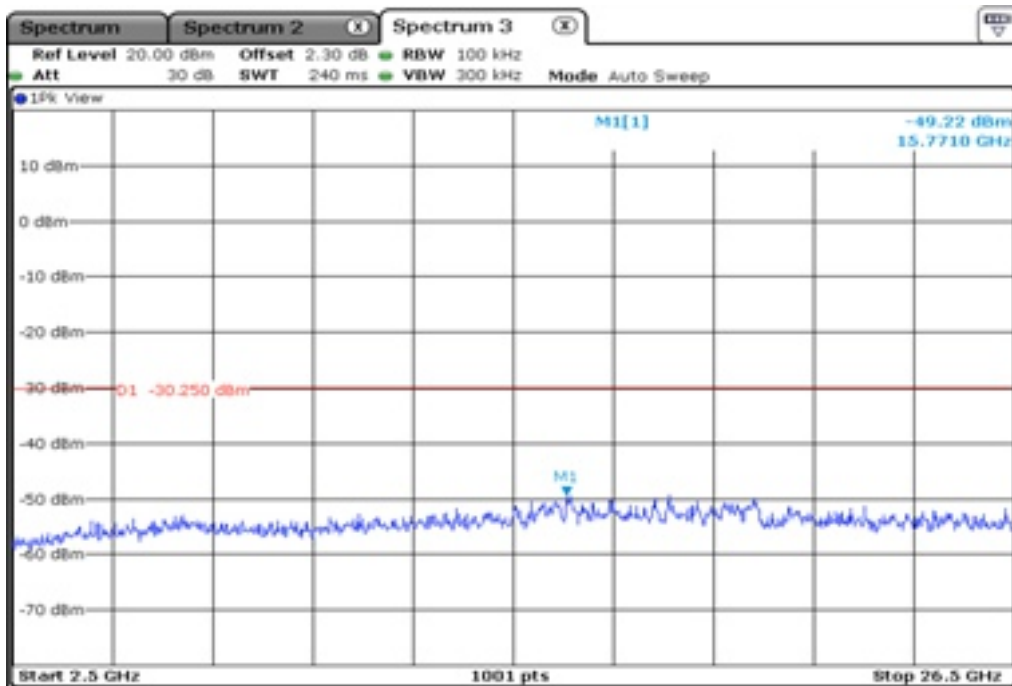
26.2 100 kHz Bandwidth
