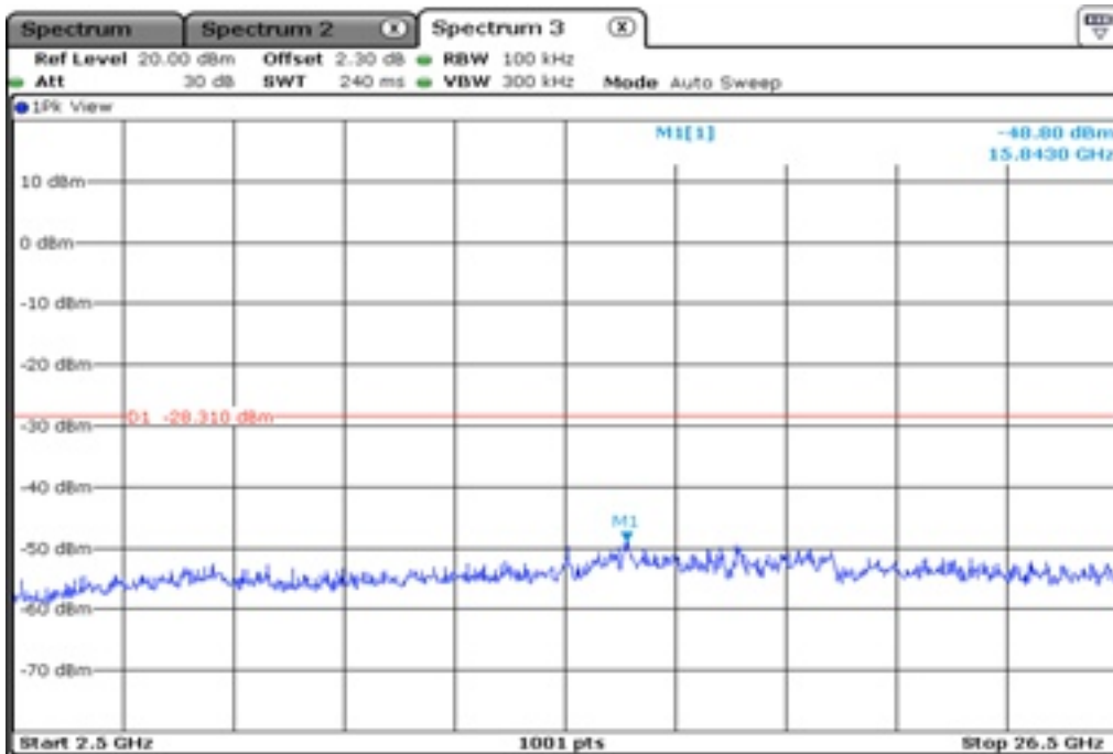
24.2 100 kHz Bandwidth
